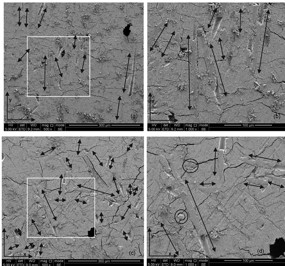
Fig. 6. Urea formaldehyde - wood flour with 10% wt glass fibres: (a) printed along the y-axis, evidence of directional alignment of fibres. (b) higher magnification image of box in Fig. 6a (c) moulded sample with randomly aligned glass fibres; small arrows indicate fibres that are almost perpendicular to analysed surface, longer arrows indicate fibres that are more parallel to analysed surface. (d) higher magnification of box in Fig. 6c moulded sample; circles indicate fibre running perpendicular to analysed surface.(a).
