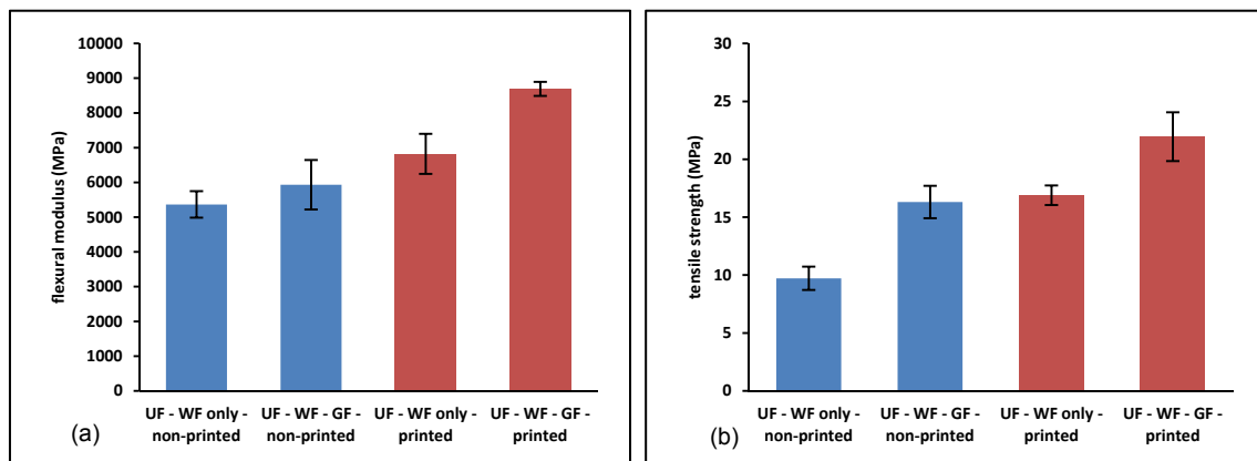
Fig. 3. Comparison of mechanical properties of printed and non-printed composites: (a) flexural modulus and (b) tensile strength. (UF = urea formaldehyde, WF = wood flour, GF = with glass fibres present).
