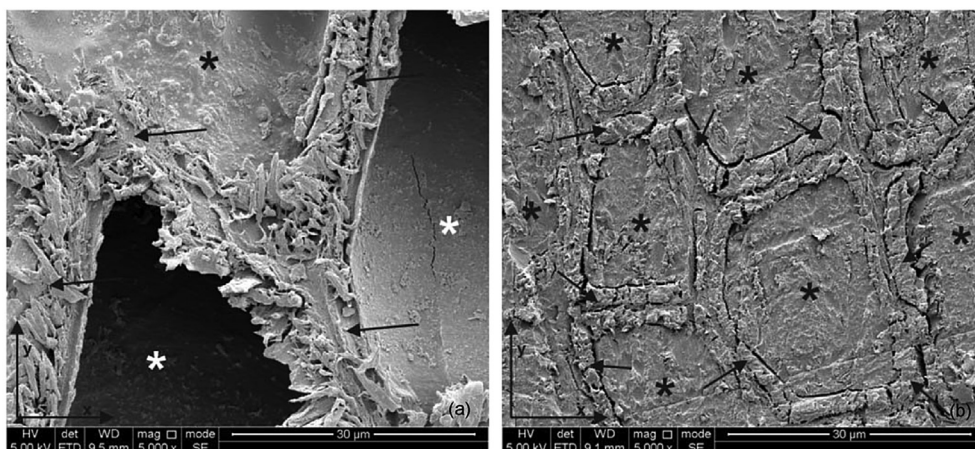
Fig. 4. Urea formaldehyde - wood flour; arrows indicate cell walls, black stars indicate UF, white stars indicate voids within the cell (a) non-printed samples (b) printed sample.
