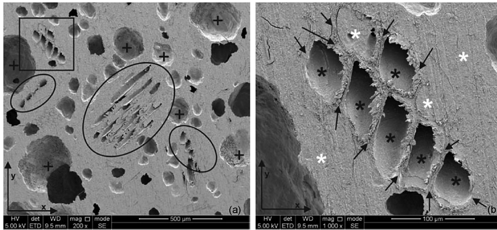
Fig. 5. Non-printed urea formaldehyde - wood flour samples: (a) wood particles indicated within circles in random orientation, + indicate gas pores. (b) Higher magnification image of box in Fig. 5a; arrows indicate wood cell wall, white stars indicate UF, black stars indicate voids within wood cell.
