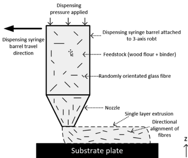
Fig. 1. Schematic of the extrusion/deposition based additive manufacturing technique and hypothesis of glass fibre alignment.
