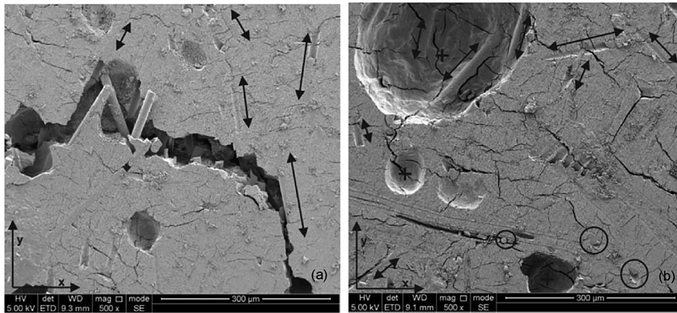
Fig. 7. Urea formaldehyde - wood flour with 10%wt glass fibres and sub-surface fibre detail: (a) printed along y-axis, densely populated and aligned fibres seen within a crack, some evidence of gas pores. (b) moulded sample with randomly aligned glass fibres, glass fibre detail shown within large gas pore.
