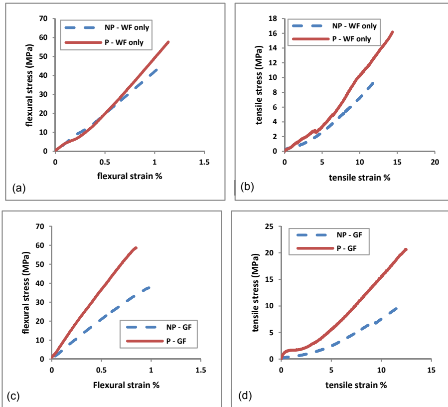
Fig. 2. Comparison of mechanical properties of printed and non-printed products: (a) flexural and (b) tensile stress strain curves for urea formaldehyde-wood flour only samples; (c) flexural and (d) tensile stress-strain curves for urea formaldehyde - wood flour - glass fibre samples. P = printed, NP = non-printed, WF = wood flour, GF = with glass fibres present.
