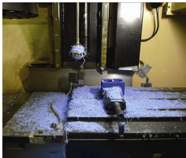
Figure 2. Cincinnati Milacron computer numerical control machine testing setup. The computer numerical control machine holds the handle which is attached to the tested reamer. The reamed cavity in the wax block is shown as well. All trials are performed in this automated manner.
