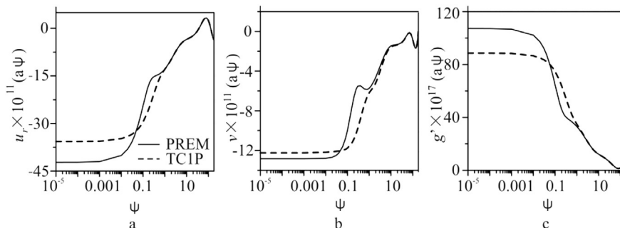
Fig. 3 – Comparison of Green's functions between TC1P and PREM models. u_r , v and g' (in cm, cm and cm/s 2 respectively) are the Green's functions for surface radial and tangential displacements, and surface gravity variation respectively. a is the Earth's radius (in cm), \psi is the angular distance (in arc) between the observer and the point mass of 1 g.
