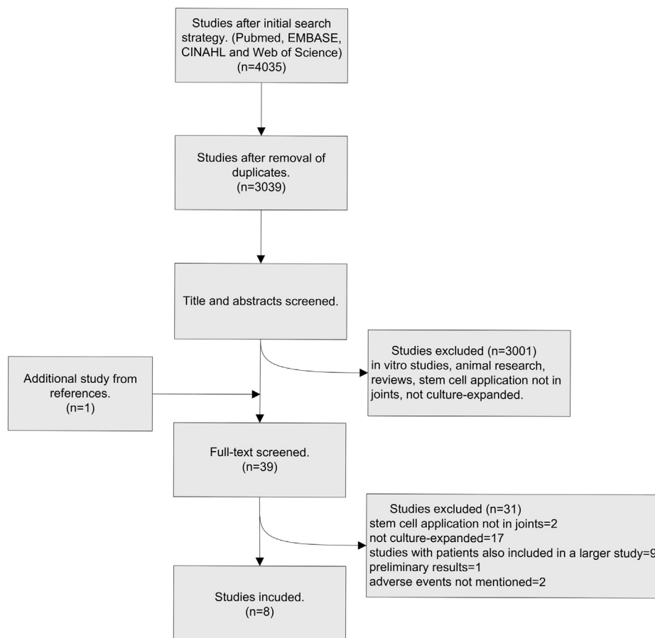
Fig. 1. Study selection.
