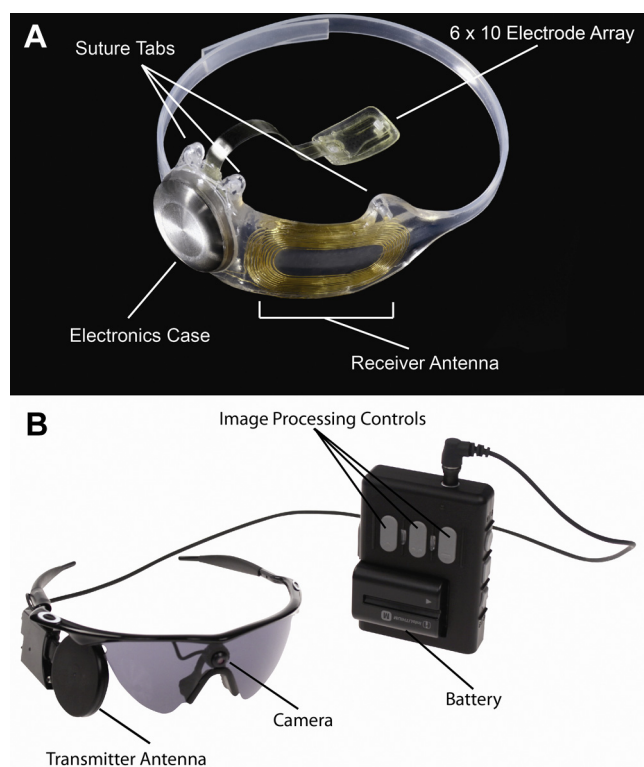
Figure 1. A , The implanted portions of the Argus II System (Second Sight Medical Products, Inc., Sylmar, CA). B , The external components of the Argus II System. Images in real time are captured by the camera mounted on the glasses. The video processing unit down-samples and processes the image, converting it to stimulation patterns. Data and power are sent via radiofrequency link from the transmitter antenna on the glasses to the receiver antenna around the eye. A removable, rechargeable battery powers the system.
