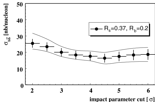
Fig. 4. Dependence of the b\bar{b} production cross section on the muon impact parameter cut. The systematic uncertainty is evaluated selecting the range [3.5\sigma, 6\sigma] , where the contribution of the prompt particle background is sufficiently small. The band represents the variation of cross section due to a change of the expected signal and background composition ( R_s and R_b ) in the ranges [0.33, 0.41] and [0.1, 0.3] , respectively.
