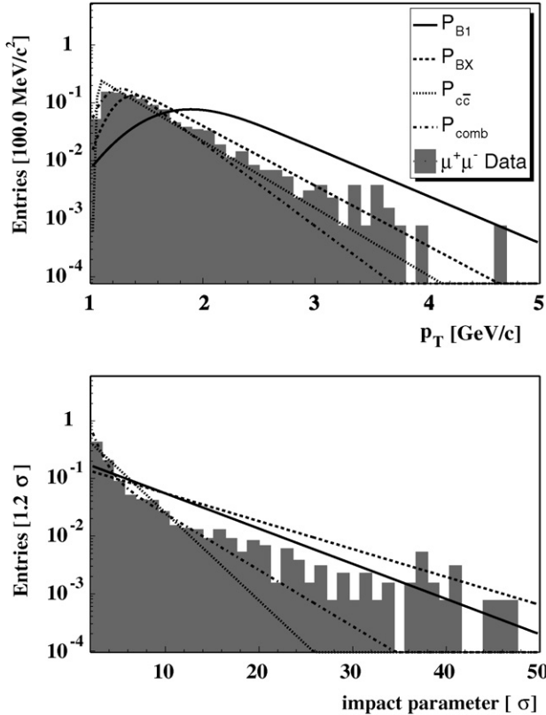
Fig. 3. Probability density functions of double muonic b and c decays and combinatorial background. The p_T (top) and I_p (bottom) distribution of unlike-sign muon events are superimposed.
