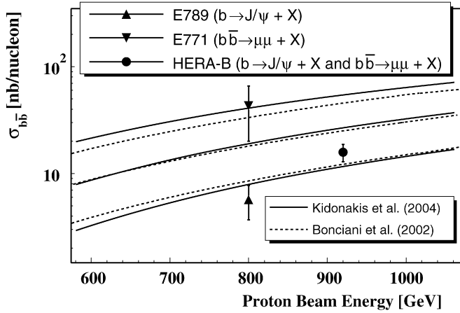
Fig. 5. Cross section for b\bar{b} production as a function of the proton energy in fixed target collisions. The predictions of Bonciani et al. [1], updated with the NNLO parton distribution function in [34], and Kidonakis et al. [2] are shown. The theoretical uncertainties are obtained by changing the renormalisation and factorisation scales and the b mass. The HERA-B result, which is based on a combined analysis of b \rightarrow J/\psi + X and b\bar{b} \rightarrow \mu\mu + X decays, is consistent with the theoretical predictions. The results of the lower energy Fermilab experiments (E771 [5] and E789 [4]) are also shown.
