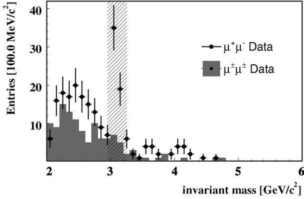
Fig. 2. Dimuon invariant mass after b\bar{b} selection. Events in the J/\psi mass region ( [2.95, 3.25] \text{GeV}/c^2 ), which is highlighted in the picture, are mostly due to b \rightarrow J/\psi + X decays. Since they are used in a different analysis [6], they are removed.
