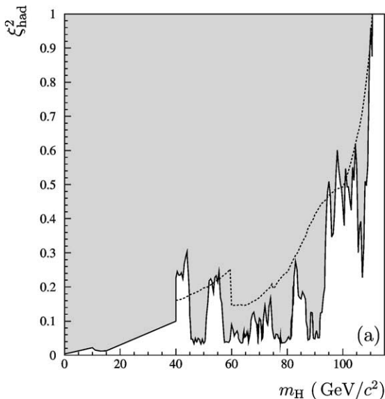
Fig. 2. Expected (dashed line) and observed (shaded area) 95% C.L. limits on (a) \xi_{\text{had}}^2 and (b) \xi_\tau^2 , as a function of the Higgs boson mass hypothesis and for centre-of-mass energies up to 209 GeV.
