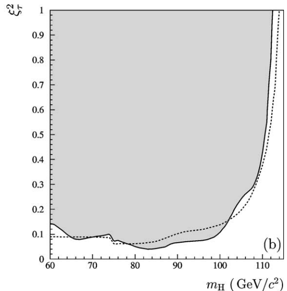
Fig. 2. Expected (dashed line) and observed (shaded area) 95% C.L. limits on (a) \xi_{\text{had}}^2 and (b) \xi_\tau^2 , as a function of the Higgs boson mass hypothesis and for centre-of-mass energies up to 209 GeV.
