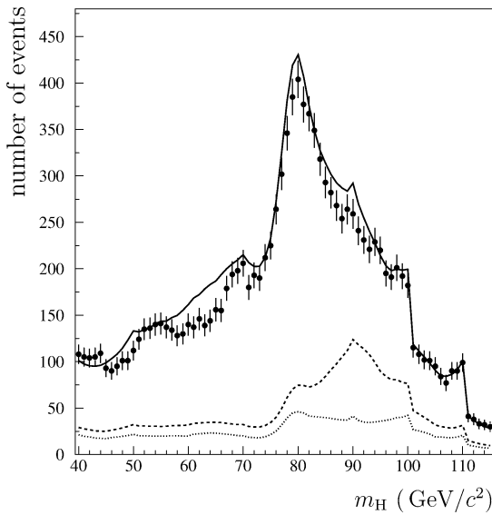
Fig. 1. Expected background (solid curve) compared to collected data (dots) by the four-jet selection as a function of the Higgs boson mass hypothesis at centre-of-mass energies from 189 to 209 GeV. The dotted curve represents the contribution from the q\bar{q} background and the dashed curve represents the additional contribution from the ZZ background.
