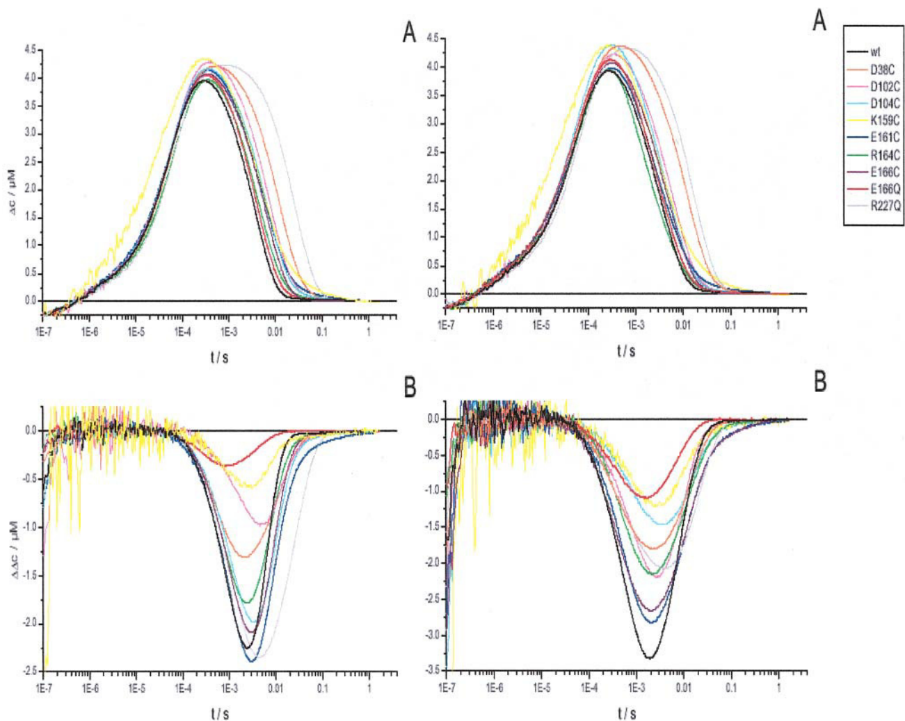
FIGURE 3 Flash-induced transient concentration changes of the M-intermediate at 412 nm (top frames) and of pyranine at 459 nm (lower frames) of WT bacteriorhodopsin and BR mutants D38C, D102C, D104C, K159C, E161C, R164C, E166C, E166Q, and R227Q ( T = 25^\circ\text{C} , \text{pH} = 7.5 ). (Left panel) The measurements were carried out in pure water. (Right panel) The measurements were carried out in 150 mM KCl.
