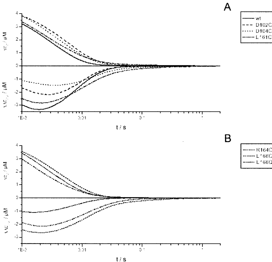
FIGURE 6 Flash-induced transient concentration changes of the M-intermediate at 412 nm ( upper traces ) and of pyranine at 459 nm of WT bacteriorhodopsin and BR mutants D102C, D104C, and E161C ( A ), and of BR mutants R164C, E166C, and E166Q ( B ), in 150 mM KCl. The measurements were carried out at T = 25^\circ\text{C} and \text{pH} = 7.5 .
