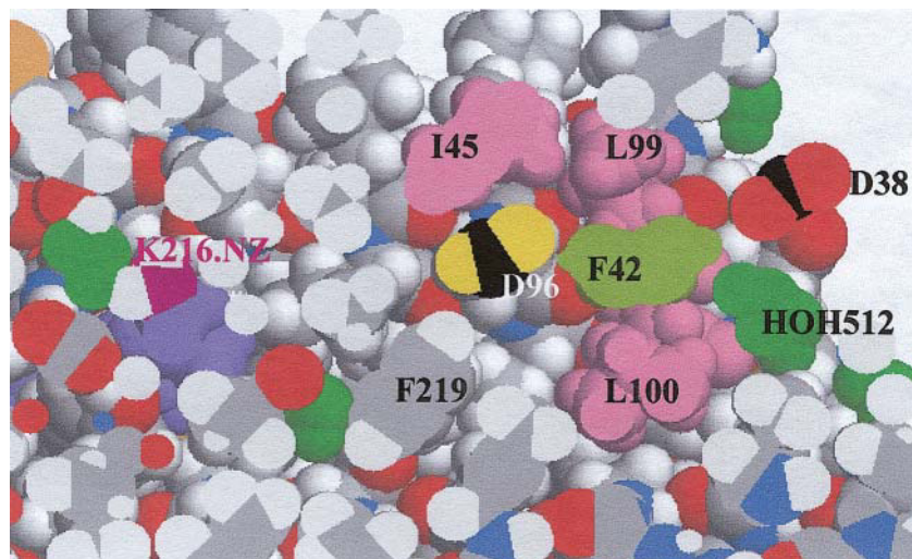
FIGURE 9 A cross-section along the bacteriorhodopsin emphasizing the trajectory of the hole propagation. The three proton-binding sites are marked in the figure. The Schiff base nitrogen ( purple ), and the carboxylates carbon atom of D96 and D38. The entrance to the hydrophobic gate is located between the carboxylate of D38 and K41 and extends over the two sides of F42 through a narrow passages between the benzene ring and the surrounding hydrophobic residues (colored in gray ) that are 4–5 Å ( center to center ) from the benzene carbons. Considering the van der Waals radii, the passages are too narrow to allow water molecules to pass through.
