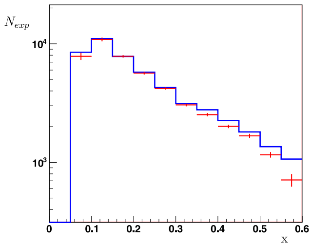
Fig. 15. x -spectrum. Red points – data, blue histogram – IB. (For interpretation of the references to color in this figure legend, the reader is referred to the web version of this Letter.)
