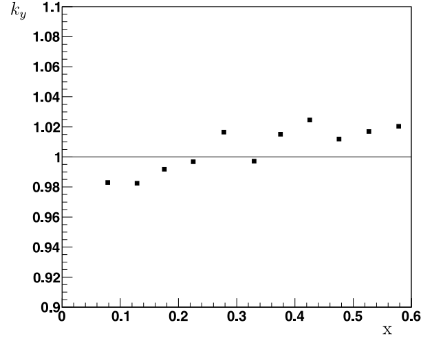
Fig. 9. Extra width k_y vs x .
