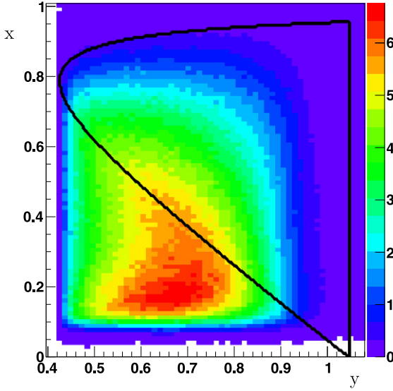
Fig. 7. Dalitz-plot density for K\mu 3 bkg.
