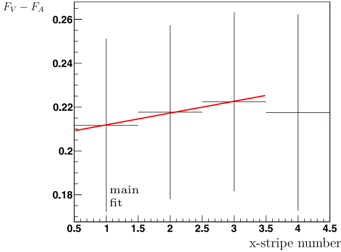
Fig. 17. Systematics of cut on x. Left border.
