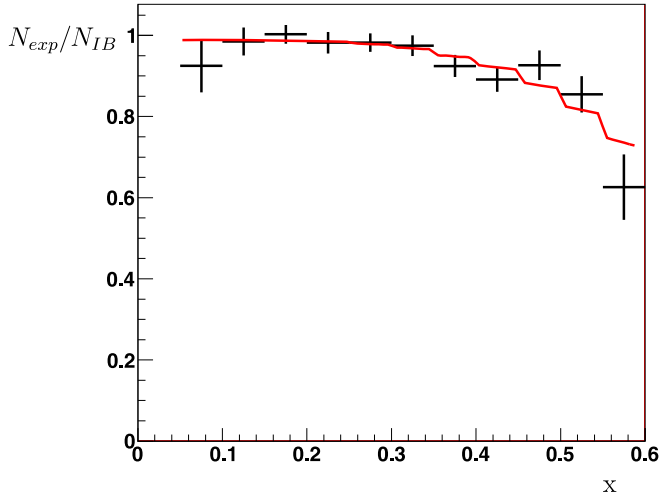
Fig. 20. \chi PT O(p^6) fit, F_V(0) and F_A taken from theory. \chi^2/\text{ndf} = 8.8/9 .
