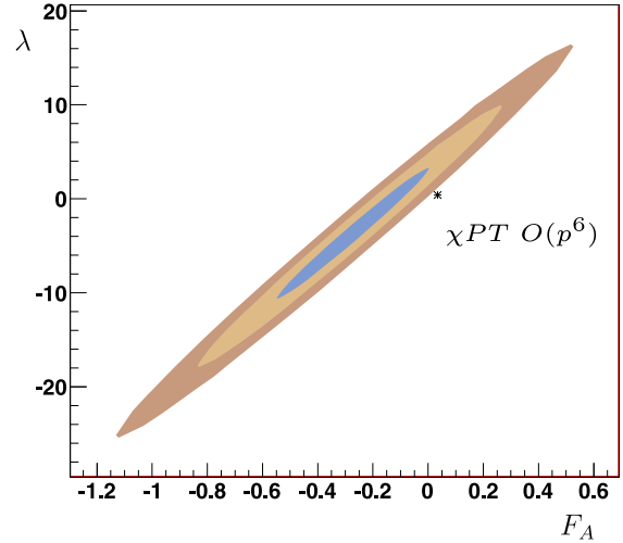
Fig. 22. \chi PT O(p^6) fit, F_V(0) taken from theory. \chi^2/\text{ndf} = 7.5/8 .
