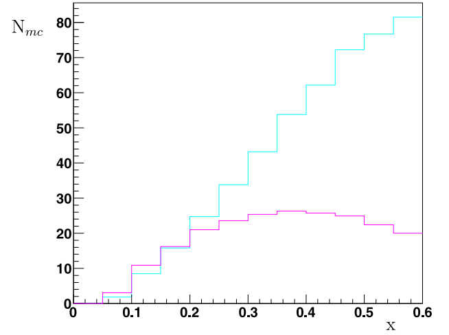
Fig. 19. \text{INT}^+ (magenta) and \text{INT}^- (cyan) contributions with F_V + F_A = 0.165 and F_V - F_A = 0.21 . (For interpretation of the references to color in this figure legend, the reader is referred to the web version of this Letter.)
