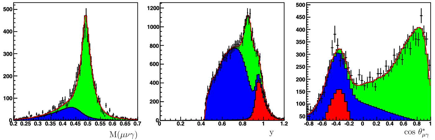
Fig. 13. Simultaneous fit in stripe 4: M(\mu\nu\gamma) , y and \cos\theta_{\mu\gamma}^* . Points with errors – data, blue – K\mu 3 , red – K\pi 2 , green – signal, red line – fit (signal + background). \chi^2/\text{ndf} = 157.3/91 (for mass histogram only, see text). (For interpretation of the references to color in this figure legend, the reader is referred to the web version of this Letter.)
