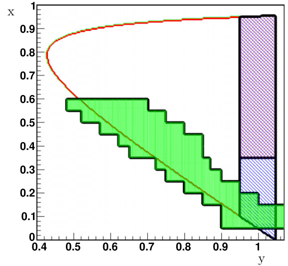
Fig. 12. ISTRA+ (green); BNL E787 (red hatch); KEK-104 (blue hatch). (For interpretation of the references to color in this figure legend, the reader is referred to the web version of this Letter.)
