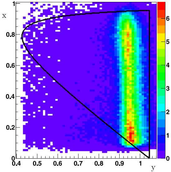
Fig. 8. Dalitz-plot density for K\pi 2 bkg.
