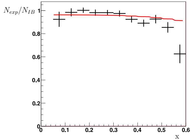
Fig. 21. LFQM fit, F_V and F_A taken from theory. \chi^2/\text{ndf} = 24.1/10 .
