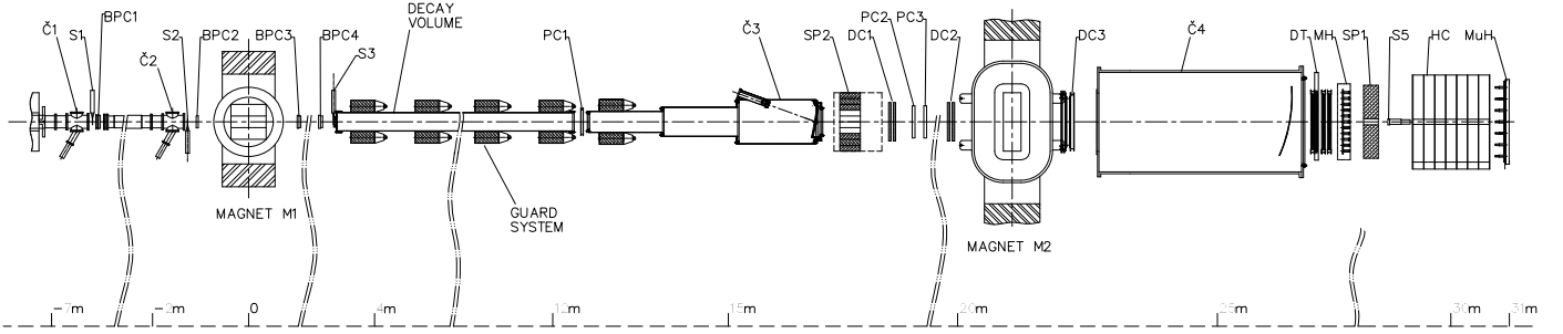
Fig. 5. Elevation view of the ISTRAP+ detector.
