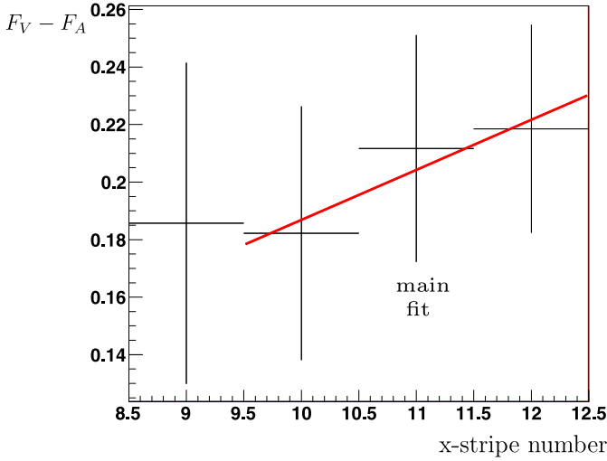
Fig. 18. Systematics of cut on x. Right border.
