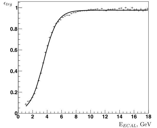
Fig. 6. T_0 trigger efficiency. Points – data, curve – fit by Fermi function.
