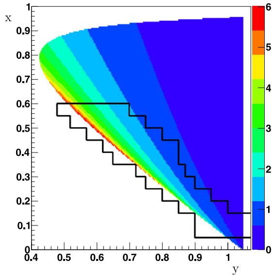
Fig. 11. \text{INT}^- Dalitz-plot density and selected kinematic region.
