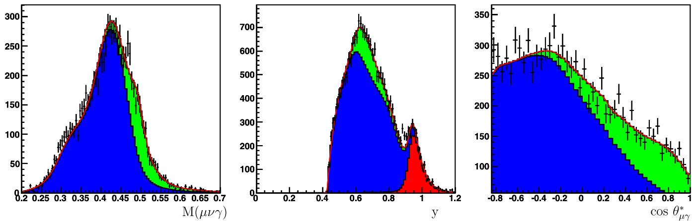
Fig. 14. Simultaneous fit in stripe 9: M(\mu\nu\gamma) , y and \cos\theta_{\mu\gamma}^* . Points with errors – data, blue – K\mu 3 , red – K\pi 2 , green – signal, red line – fit (signal + background). \chi^2/\text{ndf} = 141.7/91 (for mass histogram only, see text). (For interpretation of the references to color in this figure legend, the reader is referred to the web version of this Letter.)
