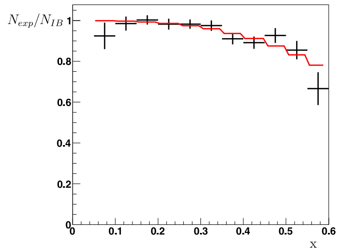
Fig. 16. N_{exp}/N_{IB} for x -stripes and final fit. \chi^2/\text{ndf} = 7.8/9 .
