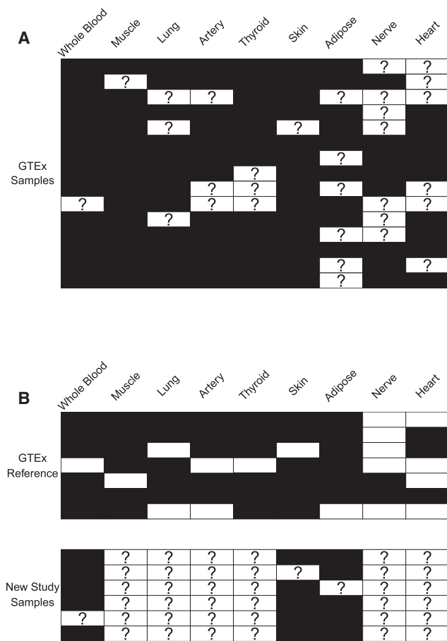
Figure 1. Illustrations of Two Imputation Scenarios In both scenarios, one can apply the proposed methods to impute the expression in the uncollected or inaccessible tissues of interest. Each row is one individual, and each column is one tissue type. The collected and measured tissues are shown in black, and the uncollected or inaccessible ones are in white. The tissues with question marks are the ones of interest. (A) Expression in the uncollected GTEx tissues (with question marks) was imputed on the basis of expression in the collected GTEx tissues. (B) Expression in the uncollected tissues (with question marks), including inaccessible tissue types, was imputed on the basis of collected tissues in a new expression study. GTEx was used as a reference.
