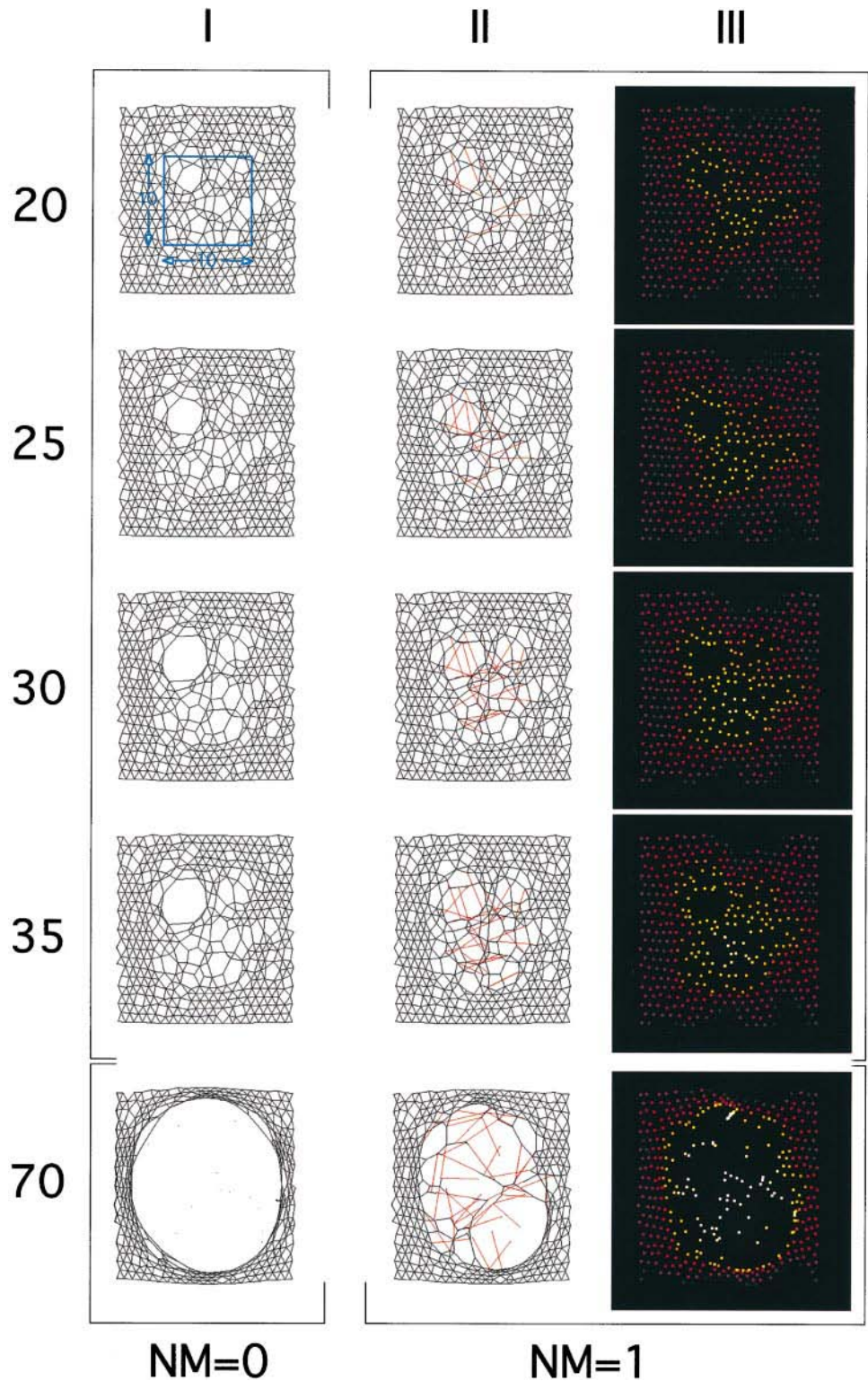
FIGURE 1 Matrix equilibrium with-out (NM = 0, first column) or with (NM = 1, second column) myosin II and weight of the junction complexes (third column). The percentage of spectrin disruption inside the blue window (upper left image) is indicated on the left of the figure and was held constant at 5% outside. In the first two columns the spectrin mesh-work is black. In the second column, actomyosin II complexes are indicated in red. The weight of the junction complex is calculated in the presence of myosin II (NM = 1, A_{min} = 0 and A_{max} = 60 ) and expressed on a gray scale ranging between 0 and 255. NM is the maximum number of MII minifilaments that may be linked to each actin protofilament.
