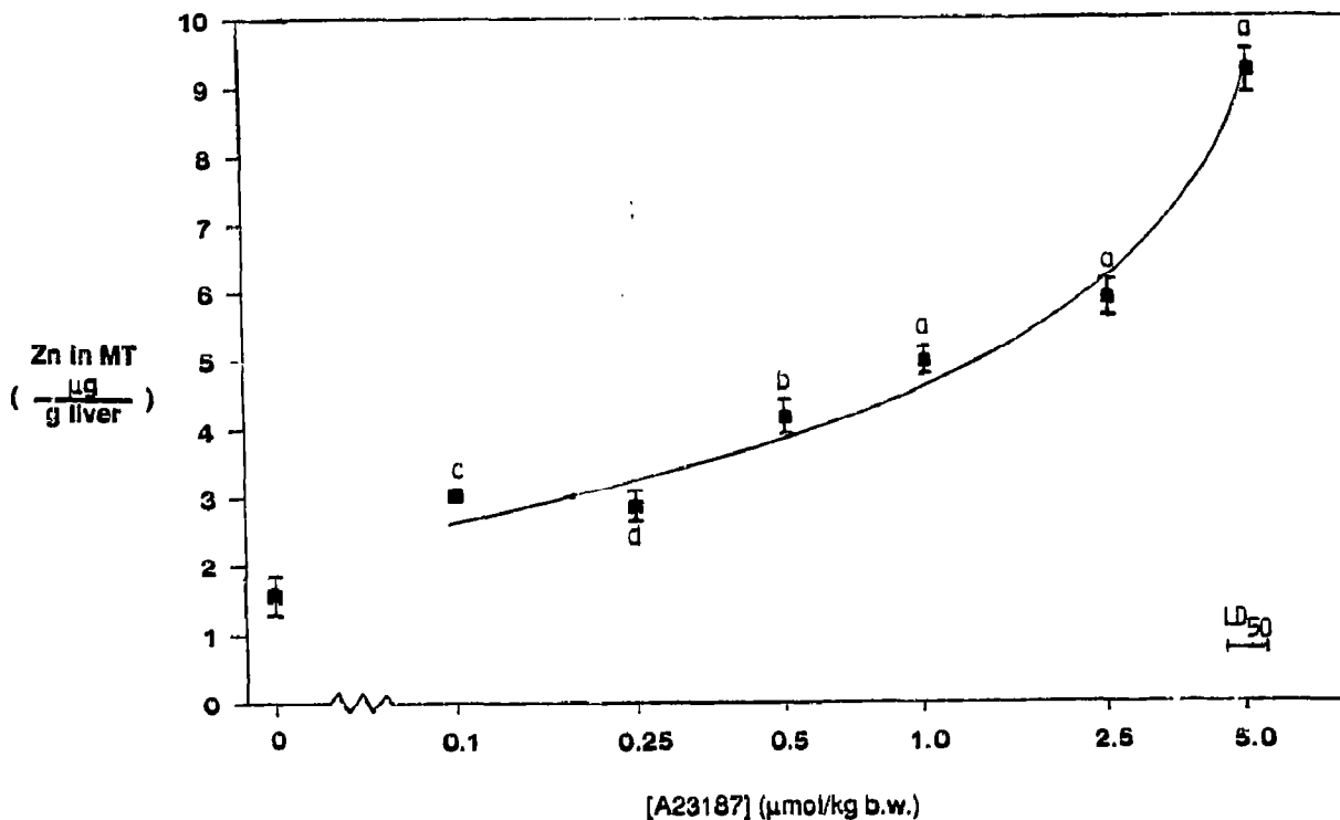
Fig. 1. A23187 dose-response for MT induction in rat liver. A23187 was administered at the indicated dosages i.p. at time 0. Animals were killed at 11 h, and MT (μg Zn/g liver) was determined by the Sephadex G-75/AAS method. The data are presented as the mean ± S.E. for at least four animals in a group. Statistically significantly different from controls (vehicle only) at a P<0.001; b P<0.01; c P<0.02, using t-test. LD 50 , lethal dose that kills 50% of the animals by 24 h, as reported by the manufacturer. No animal in these groups died during the 11 h treatment period.
