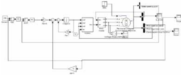
Fig. 1 Simulation model of PMSM system which uses traditional PID controller
