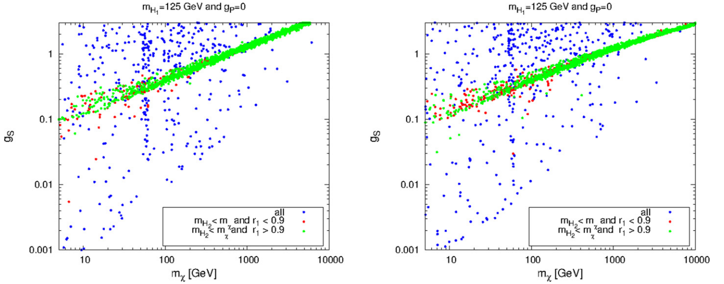
Fig. 3. Parameter choices giving rise to a relic density in the WMAP range in the Higgs portal model with m_{H_1} = 125 GeV and g_p = 0 . Green and red points correspond to m_{H_2} < m_\chi with a more ( r_1 > 0.9 ) or less ( r_1 < 0.9 ) SM Higgs-like H_1 , respectively. We show the scalar coupling g_S as a function of the dark matter mass without (left) and with (right) Sommerfeld enhancement for the relic density computation. For illustration, we also show the points with m_{H_2} > m_\chi (blue points). (For interpretation of the references to color in this figure legend, the reader is referred to the web version of this Letter.)
