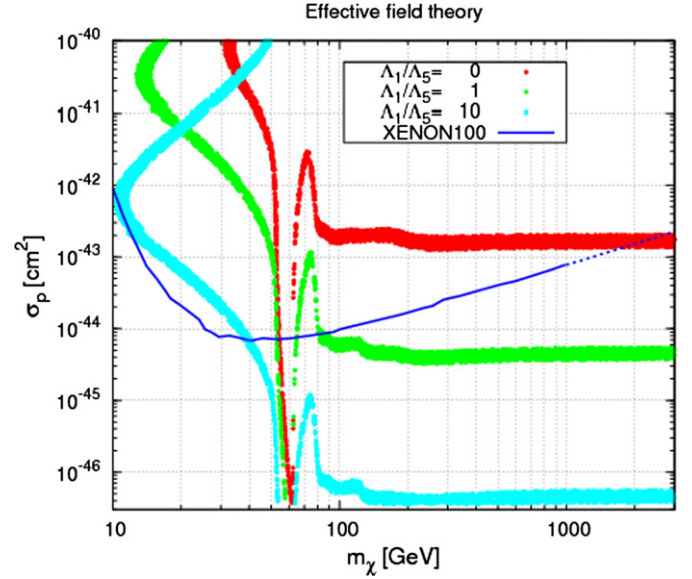
Fig. 1. Proton–dark matter scattering cross section as a function of the dark matter mass in the effective field theory of Eq. (2), as predicted by requiring that the correct relic density is obtained by thermal freeze-out. The scattering cross section is shown for several ratios of pseudo-scalar coupling to scalar coupling \Lambda_1/\Lambda_5 , and compared to the limit from XENON100 [19].
