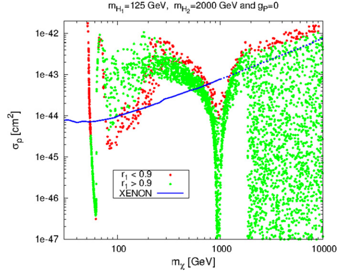
Fig. 2. Proton-DM scattering cross section as a function of the dark matter mass in the Higgs portal model for m_{H_1} = 125 GeV, m_{H_2} = 2 TeV, and g_P = 0 . The green points correspond to a SM-like H_1 with an LHC Higgs signal strength modifier r_1 > 0.9 , while the red points have r_1 < 0.9 . The points above the blue line are excluded at 95% CL by the XENON100 experiment [19]. This exclusion limit has been extended for m_\chi > 1 TeV assuming a linear dependence in m_\chi . (For interpretation of the references to color in this figure legend, the reader is referred to the web version of this or Letter.)
