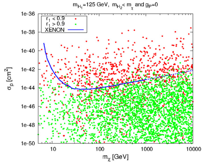
Fig. 4. Parameter choices giving rise to a relic density in the WMAP range in the Higgs portal model with m_{H_1} = 125 GeV and g_p = 0 . Green and red points correspond to m_{H_2} < m_\chi with a more ( r_1 > 0.9 ) or less ( r_1 < 0.9 ) SM Higgs-like H_1 , respectively. We show the DM–proton scattering cross section as a function of the dark matter mass for m_{H_2} < m_\chi only. The points above the blue line are excluded at 95% CL by the XENON100 experiment [19]. This exclusion limit has been extended for m_\chi > 1 TeV assuming a linear dependence in m_\chi . (For interpretation of the references to color in this figure legend, the reader is referred to the web version of this Letter.)
