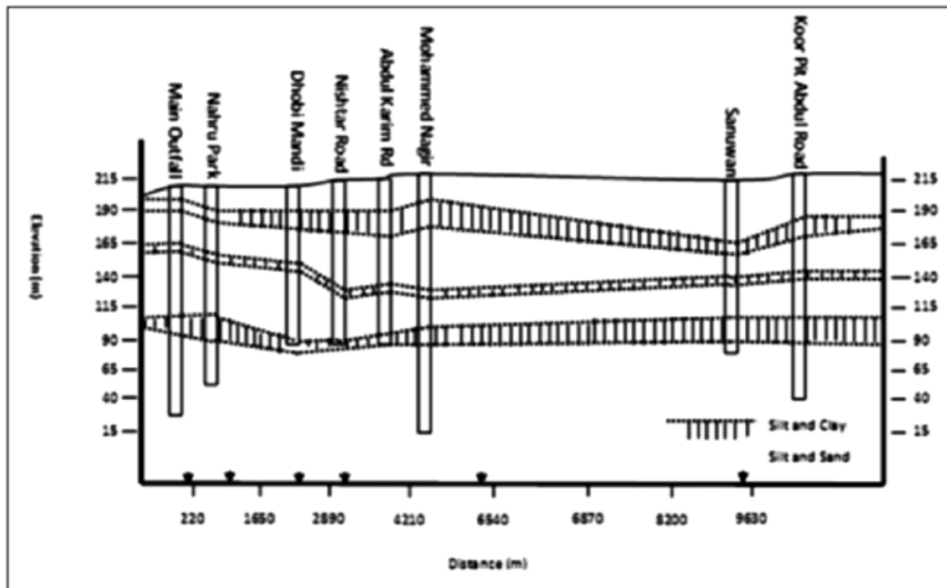
Figure 2. Geological structure of the Lahore aquifer (Source: Niaz, 2005).
