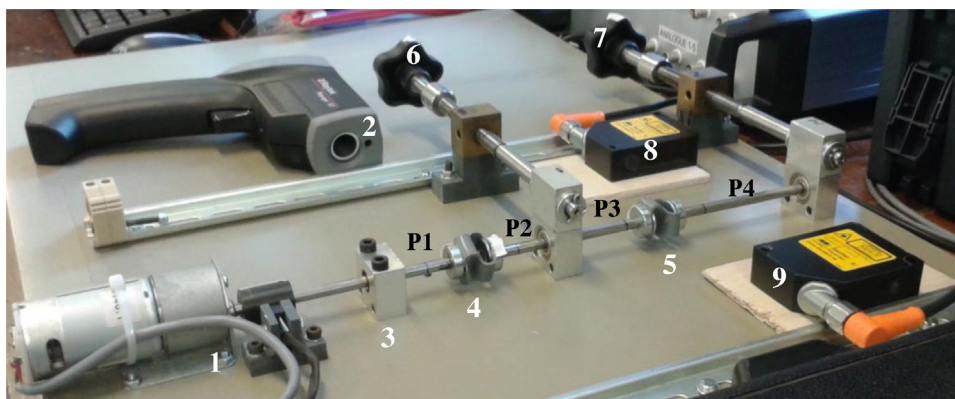
1-DC Motor 2-Infrared Thermometer 3-Fixed Bearing 4-Coupling1 5-Coupling2 6-Lead Screw1 with bearing 7-Lead Screw2 with Bearing 8-Left Measurement Laser 9-Right Measurement Laser
