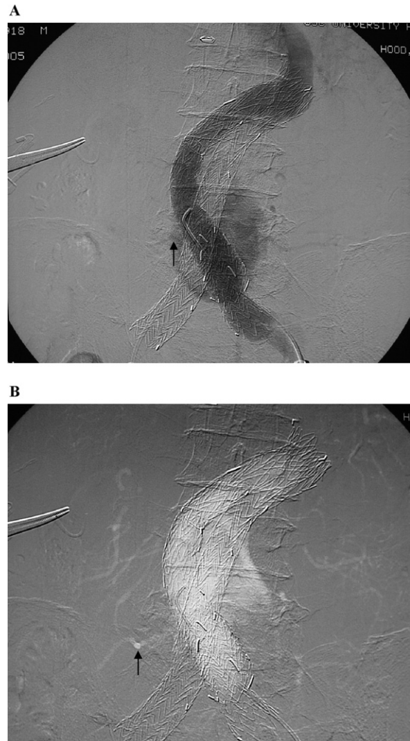
Fig 3. Type II endoleak intraoperatively documented by (A) iodinated contrast and (B) carbon dioxide digital subtraction angiography. Arrows point to feeding lumbar arteries.
