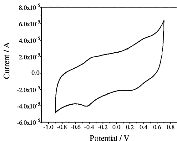
Fig. 2. Cyclic voltammogram on an edge-plane graphite electrode of SCF-K344C modified with N -ferrocenyl maleimide (12 \mu M) in 50 mM Tris-HCl pH 7.4 containing 1 mM D-(+)-camphor and 300 mM KCl at a scan rate of 10 V s -1 at 298 K.
