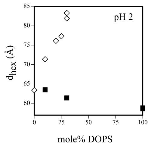
FIGURE 9 Equilibrium lattice dimensions of hexagonal phases formed at pH 2 by various DOPE/DOPS mixtures; (◇) with tetradecane, and (■) without tetradecane.
