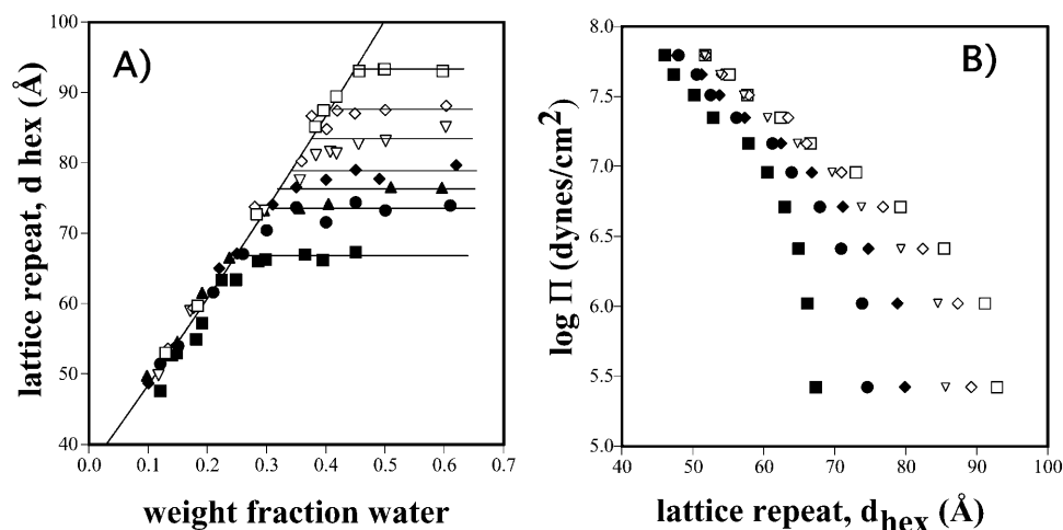
FIGURE 3 (A) Lattice dimension, d_{\text{hex}} , as it varies with water content, for the hexagonal phases formed by various DOPE/DOPS/td mixtures. Symbols are ( \square ) 30%, ( \diamond ) 25%, ( \nabla ) 20%, ( \blacklozenge ) 15%, ( \blacktriangle ) 10%, ( \bullet ) 8%, and ( \blacksquare ) 0% DOPS. Horizontal lines at equilibrium dimensions were drawn using the relationship found in Fig. 2. (B) Lattice dimension, d_{\text{hex}} , for the mixtures in A, as it varies with osmotic pressure \Pi , generated by PEG solutions of known osmotic pressure. Symbols as in A.
