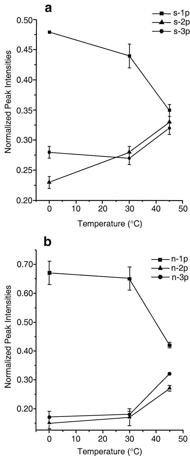
Figure 5. Average normalized mass spectral peak intensities plotted as a function of polymerization temperature: sec-butyllithium initiated polymerization (a) and n-butyllithium initiated polymerization (b).
