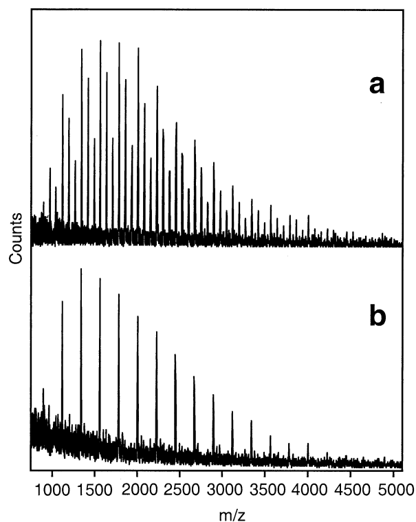
Figure 1. Positive ion spectra for sec-butyllithium (a) and n-butyllithium (b) initiated polymerizations of PDMS.
