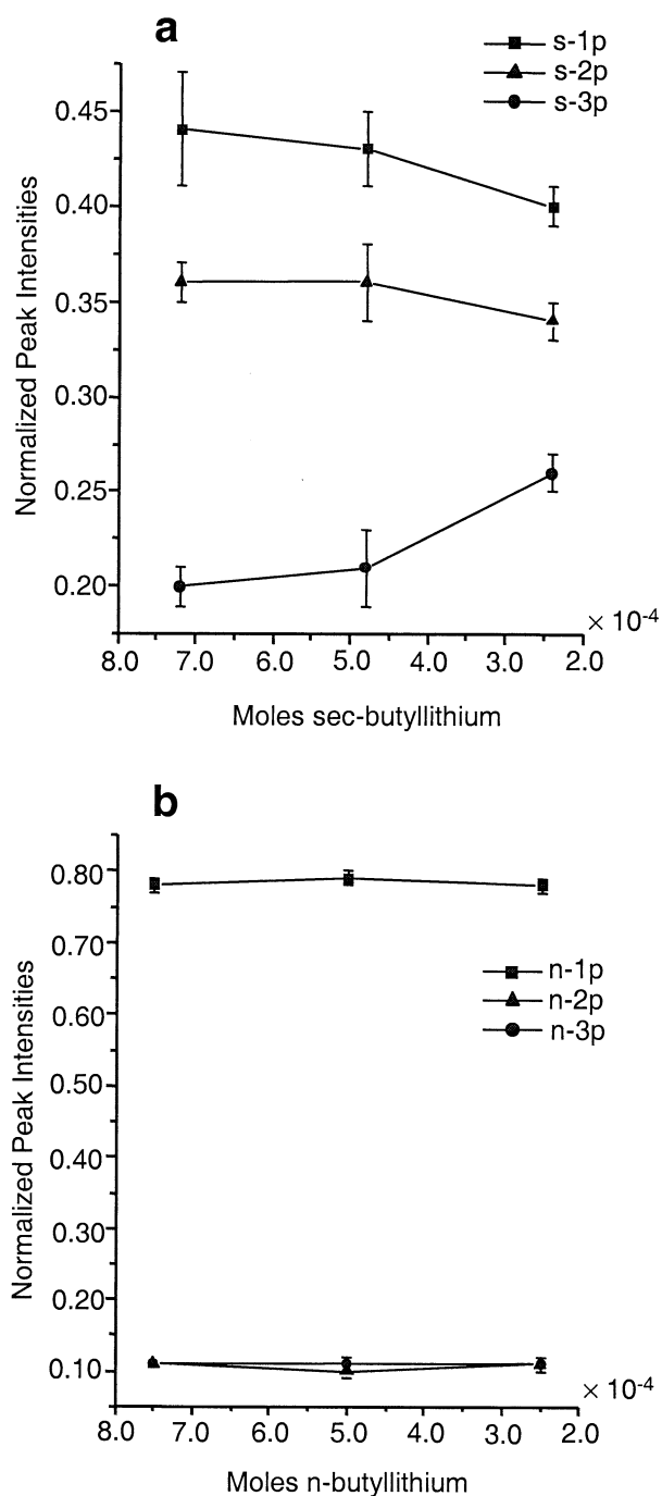
Figure 4. Average normalized mass spectral peak intensities plotted as a function of butyllithium concentration: sec-butyllithium initiated polymerization (a) and n-butyllithium initiated polymerization (b).
