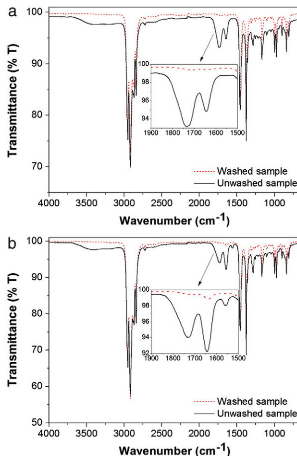
Fig. 5. FTIR spectra of PP treated at 60 Hz and 17 kHz DBD using the same energy dose of 20 J/cm 2 with discharge frequency of (a) 60 Hz and (b) 17 kHz.
