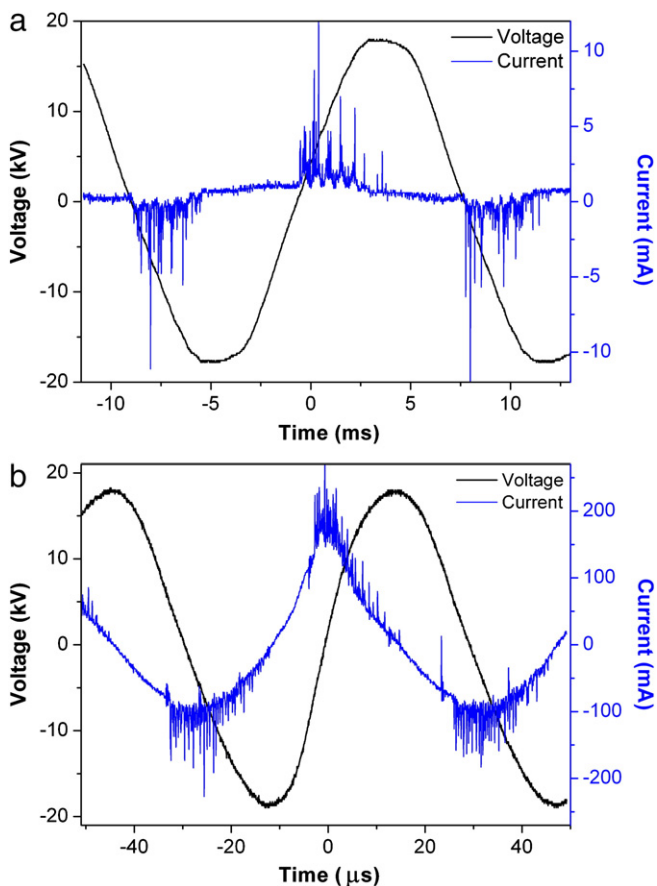
Fig. 2. Typical current and voltage waveforms for (a) 60\text{ Hz} and (b) for 17\text{ kHz} DBD.
