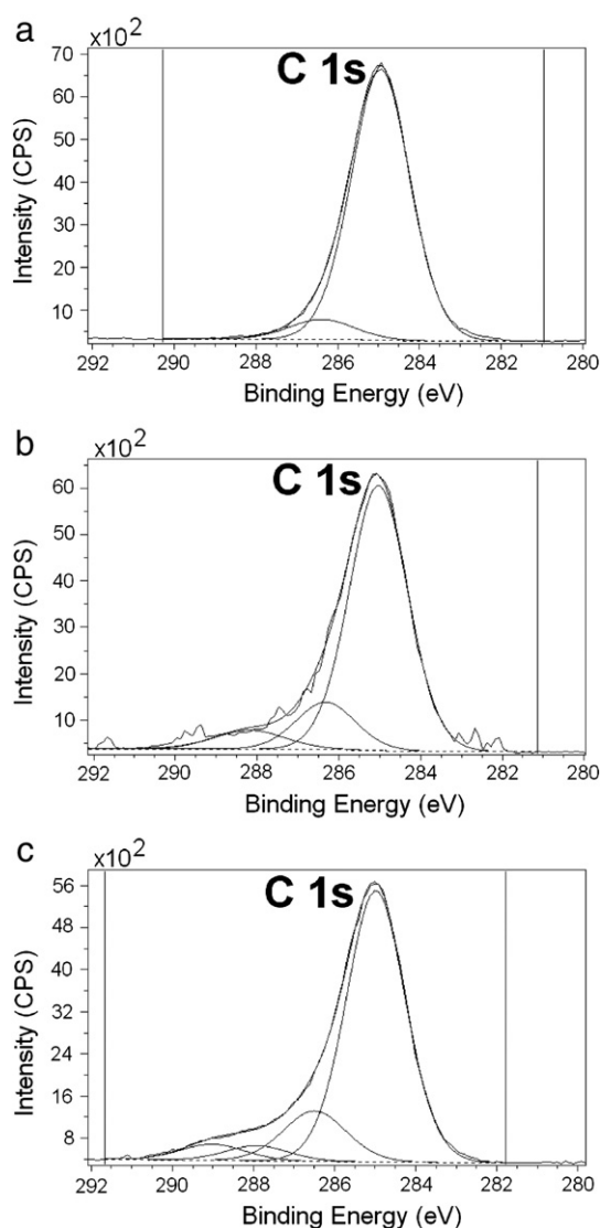
Fig. 4. Carbon C1s XPS spectra of (a) untreated PP and plasma-treated samples at 20 J/cm 2 with frequency of (b) 60 Hz and (c) 17 kHz.
