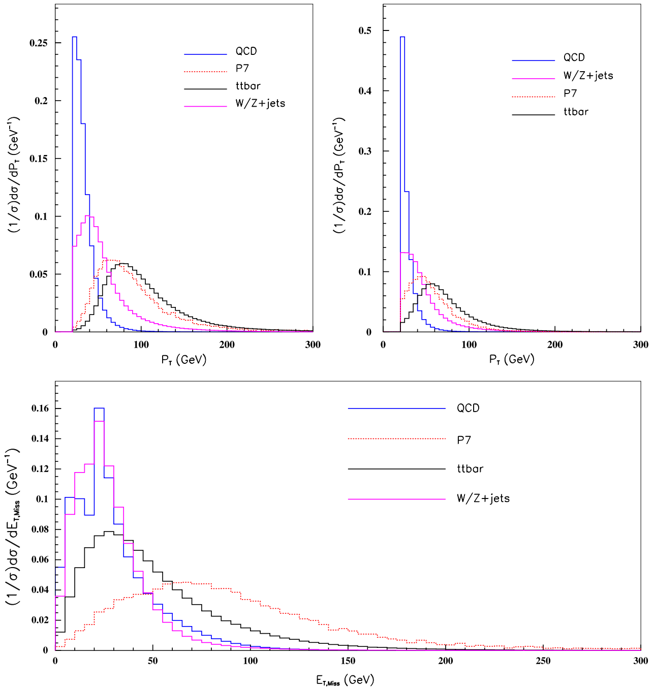
Fig. 1. Normalized p_T distributions of two highest p_T jets (upper panels) and normalized missing E_T distributions of signal and SM backgrounds (lower panel). In the figures, P7 denotes signal with R^{-1} = 700 GeV and \Delta R = 10 .
