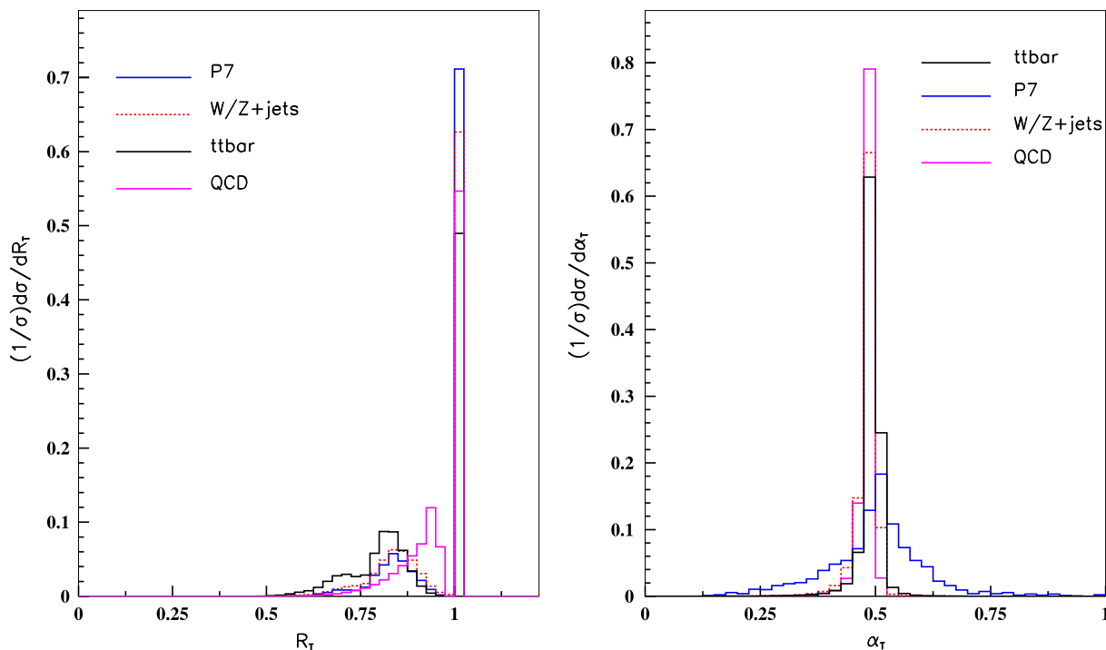
Fig. 2. Normalized R_T (left panel) and \alpha_T (right panel) distributions of signal and SM backgrounds. In the figures, P7 denotes signal with R^{-1} = 700 GeV and \Delta R = 10 .
