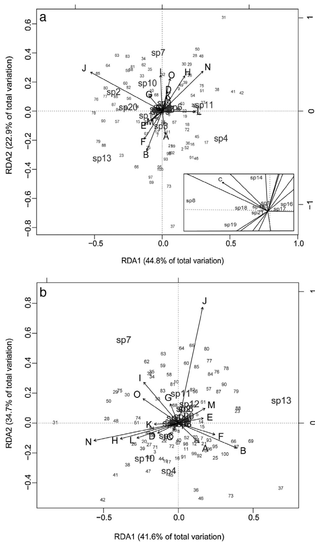
Fig. 4. Redundancy analysis ordination for dung beetle abundance (a) and biomass (b) constrained by environmental variables. Triplot with explanatory variables, species and samples: sp. 1: Bdelyrus braziliensis ; sp. 2: Canthidium aff. trinodosum ; sp. 3: Canthon luctuosus ; sp. 4: Canthon rutilans cyanescens ; sp. 5: Canthonella aff. intriata ; sp. 6: Coprophanaeus dardanus ; sp. 7: Coprophanaeus saphirinus ; sp. 8: Deltochilum brasiliense ; sp. 9: Deltochilum furcatum ; sp. 10: Deltochilum morbillosum ; sp. 11: Deltochilum multicolor ; sp. 12: Deltochilum rubripenne ; sp. 13: Dichotomius sericeus ; sp. 14: Dichotomius quadrinodosus ; sp. 15: Dichotomius sp.; sp. 16: Eurysternus cyanescens ; sp. 17: Eurysternus parallelus ; sp. 18: Paracanthion aff. rosinae ; sp. 19: Phanaeus splendidulus ; sp. 20: Uroxys sp. 1; sp. 21: Uroxys sp. 2; A: basal area of first tree; B: height of first tree; C: top diameter of first tree; D: distance to first tree; E: basal area of first shrub; F: height of first shrub; G: top diameter of first shrub; H: distance to first shrub; I: land slope; J: altitude; K: leaf litter cover; L: green cover; M: exposed soil; N: height of leaf litter; O: canopy cover; 1–25: ANH sampling points; 26–50: ITA sampling points; 51–75: PER sampling points; 76–100: RAT sampling points.
