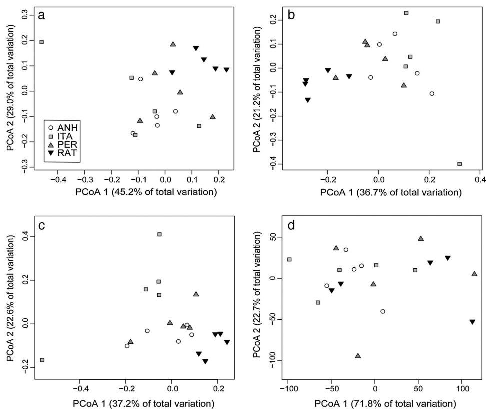
Fig. 2. Principal coordinates analysis (PCoA) of dung beetle species based on Bray–Curtis similarity and environmental variables based on Euclidean distance. The analysis was performed using presence–absence (a), abundance (b) and biomass (c) data of dung beetles, and 15 environmental variables (d). ANH: Anhatomirim Environmental Protection Area; ITA: Permanent Protection Areas of Itapema; PER: Peri Lagoon Municipal Park; RAT: Permanent Protection Areas of Ratones.
