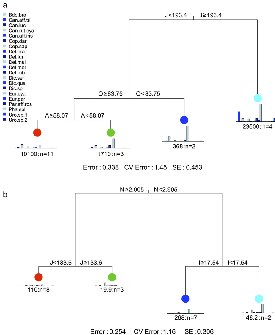
Fig. 3. Multivariate Regression Tree (MRT) analysis of the dung beetle abundance (a) and biomass with environmental variables as predictor variables. Environmental variables: A, basal area of trees; l, land slope; J, altitude; N, height of leaf litter; O, canopy cover. Species names are abbreviated and can be found in legend of Fig. 4 and in Appendix C. Bar charts at the terminal leaves of the regression tree represent species abundance means. The order of bars in each bar chart are the same and follows the sequence of names showed at left.
