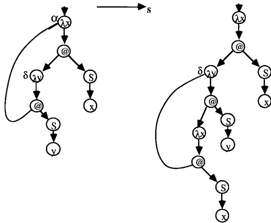
FIG. 20. Display of a substitution step.
