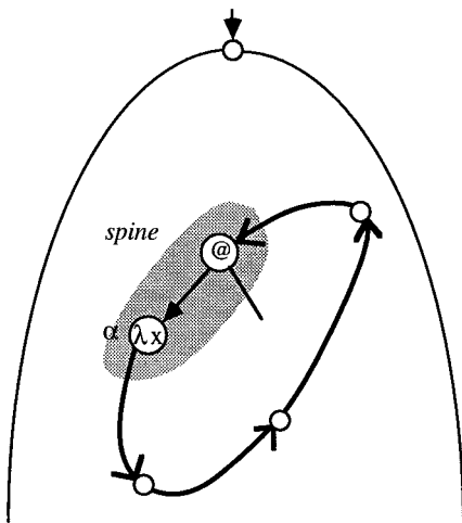
FIG. 17. Cycle through a spine.
