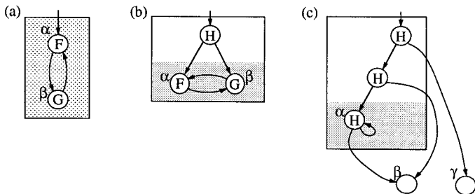
FIG. 21. Graphs associated to \lambda\phi -terms.
