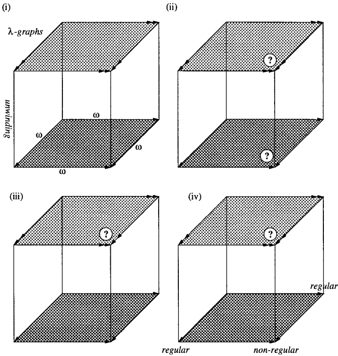
FIG. 15. Relation between \lambda -graph and \lambda -tree reductions.
