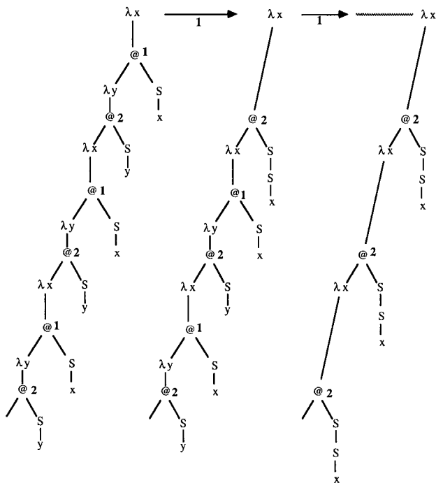
FIG. 12. Complete development of the redexes marked as 1.
