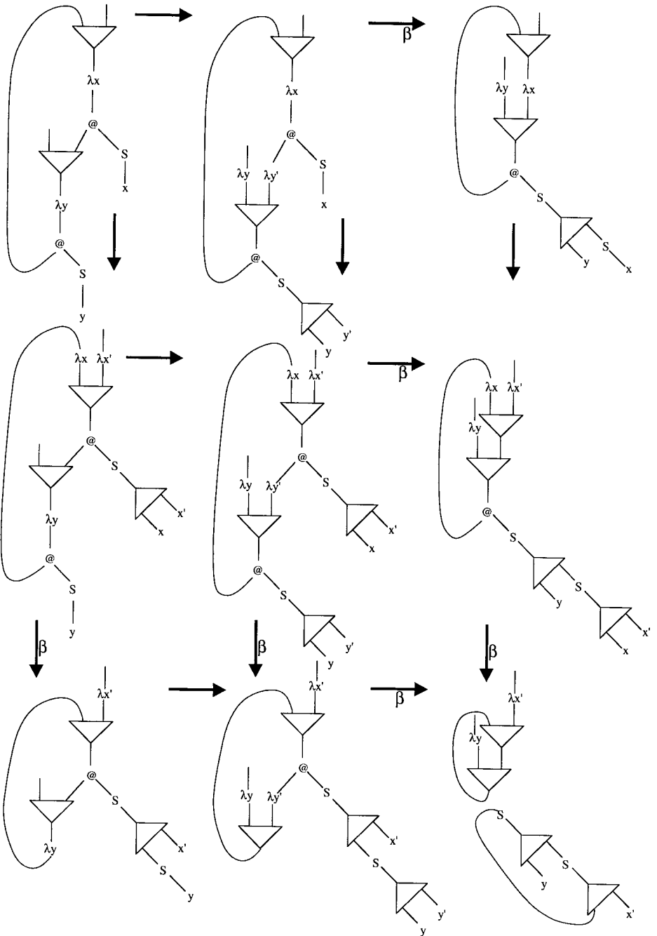
FIG. 38. First counterexample in interaction nets.
