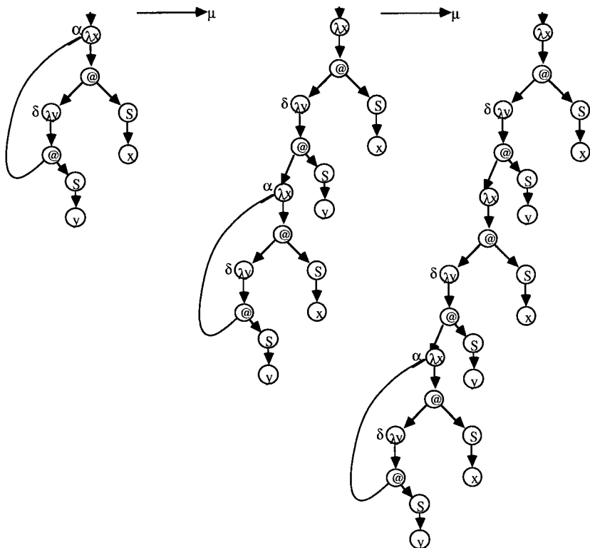
FIG. 19. \mu -reduction of \mu\alpha.\lambda x.(\mu\delta.\lambda y.\alpha(Sy))(Sx) .
