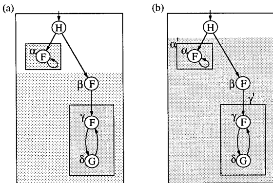
FIG. 22. Graphs associated to \lambda\phi -terms.
