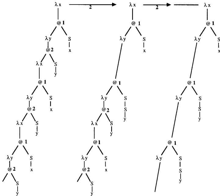
FIG. 13. Complete development of the redexes marked as 2.
