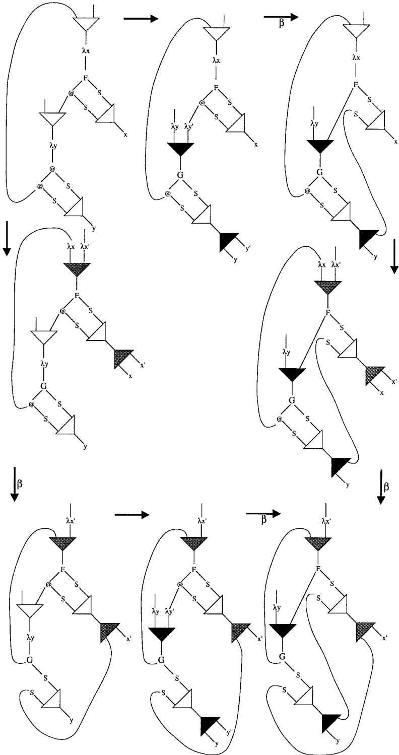
FIG. 39. Third counterexample in interaction nets.
