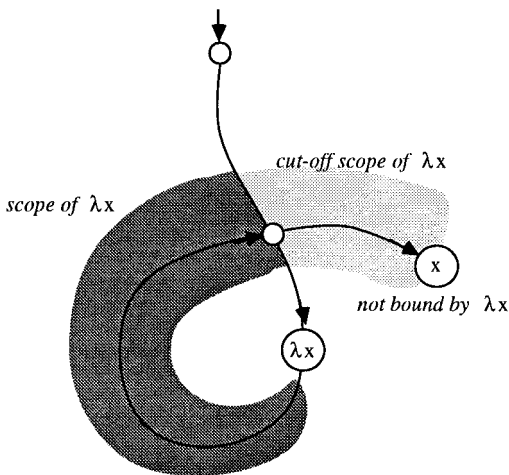
FIG. 7. Scope cut-off phenomenon.
