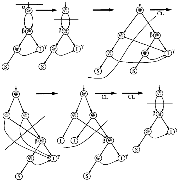
FIG. 25. Reduction in \lambda\phi_0 \cup R .
