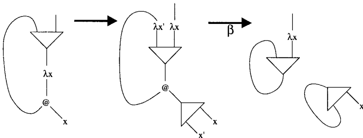
FIG. 36. Fan-in and \lambda -reduction.
