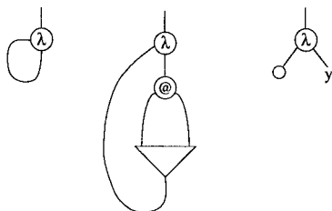
FIG. 30. Interaction nets for \lambda x.x , \lambda x.xx , and \lambda x.y .
