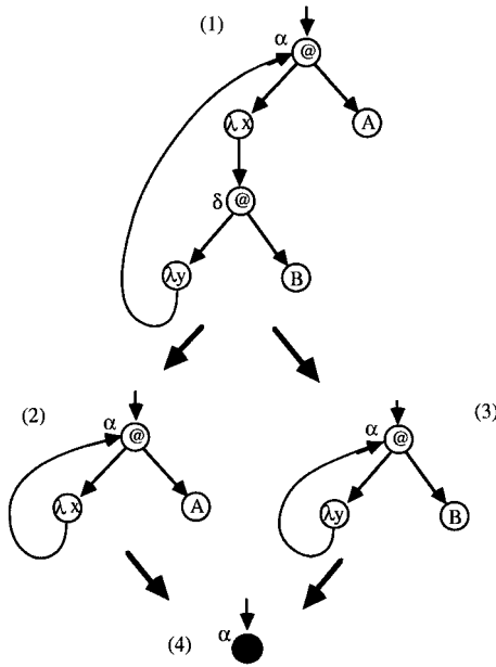
FIG. 9. Reductions to black hole.
