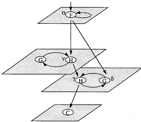
FIG. 16. Ordering among recursion variables.
