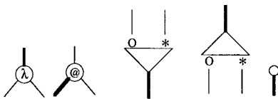
FIG. 29. Nodes of an interaction net for \lambda -calculus.
