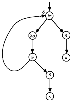
FIG. 6. Cyclic lambda graph corresponding to \delta = (\lambda x. F(\delta, Sx))(Sx) .
