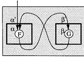
FIG. 23. Mutually dependent cyclic boxes.
