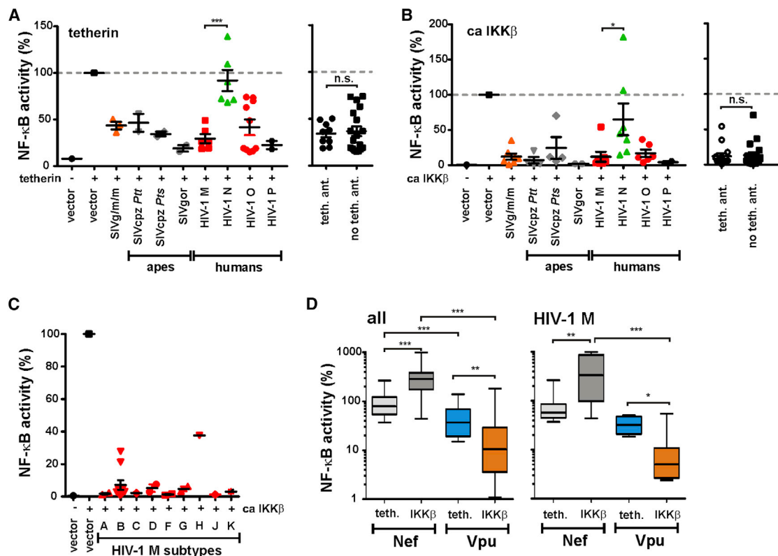
Figure 3. Inhibition of NF-κB Activation by Vpu
