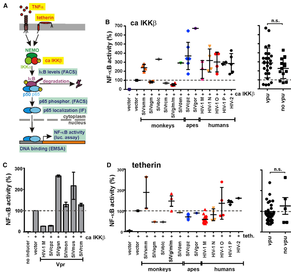
Figure 1. Stimulation of NF- \kappa B Activity by Primate Lentiviral Nef Proteins
