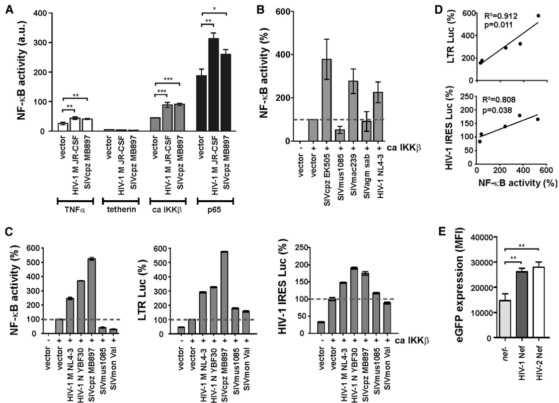
Figure 2. Primate Lentiviral Nef Proteins Stimulate Viral LTR Activity
