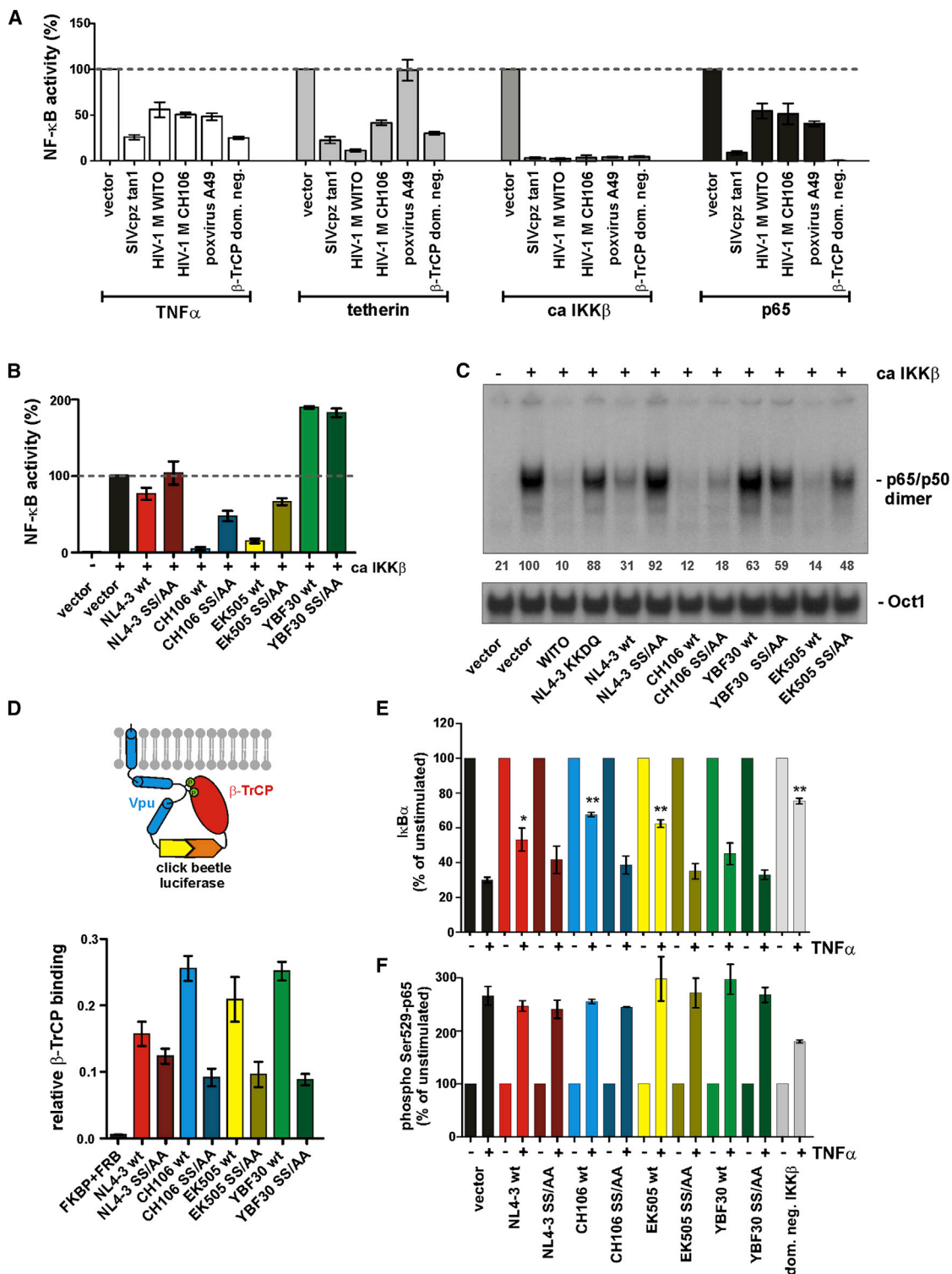
Figure 4. Mechanism of Vpu-Mediated Inhibition of NF-κB Activation
