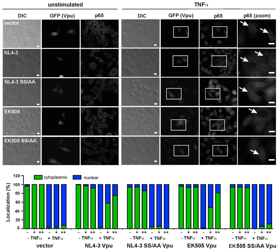
Figure 5. Vpu Inhibits Nuclear Translocation of p65
