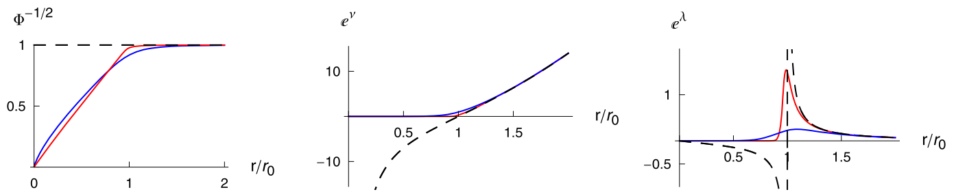
Fig. 2. The configuration e^\lambda , e^\nu and \phi with \Lambda < 0 and k = 0 . The parameters are set as a = 0.05 and L = 1 . The blue and red lines refer to the expansion parameters s = 0.1 and 0.01 . The dashed lines depict the usual BH solutions with s = 0 . (For interpretation of the references to color in this figure legend, the reader is referred to the web version of this Letter.)
