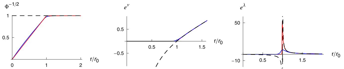
Fig. 1. The configuration e^\lambda , e^\nu and \phi with \Lambda < 0 and k = 1 . The parameter in scalar potential and the AdS radius are fixed as a = 0.1 and L = 2 . The blue and red lines refer to the expansion parameters s = 0.1 and 0.01 . The dashed lines depict the usual BH solutions with s = 0 . (For interpretation of the references to color in this figure legend, the reader is referred to the web version of this Letter.)
