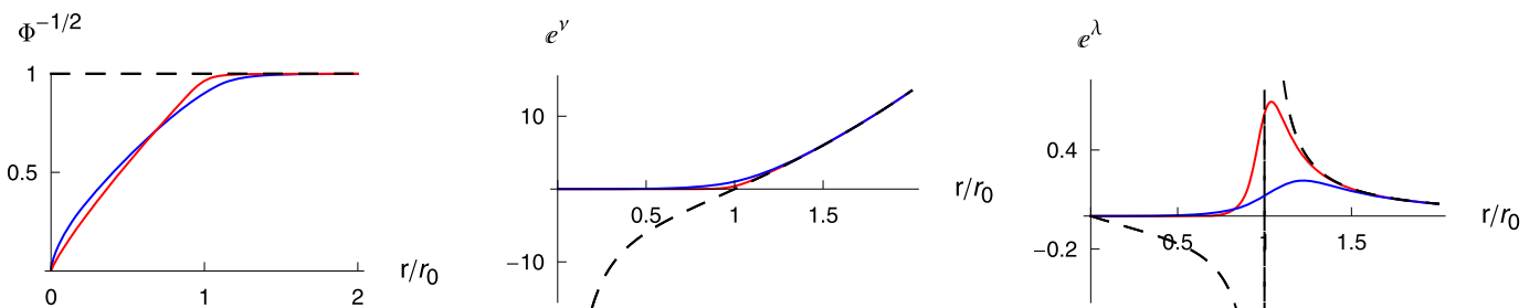
Fig. 3. The configuration e^\lambda , e^\nu and \phi with \Lambda < 0 and k = -1 . The parameters are set as a = 0.01 and L = 0.5 . The blue and red lines refer to the expansion parameters s = 0.1 and 0.01 . The dashed lines depict the usual BH solutions with s = 0 . (For interpretation of the references to color in this figure legend, the reader is referred to the web version of this Letter.)
