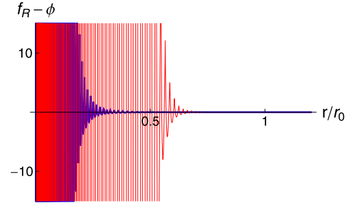
Fig. 5. Check of the condition f_R = \phi for the core with Schwarzschild exterior. The parameter a = 0.01 . The blue and red lines refer to s = 0.1 and 0.01 . (For interpretation of the references to color in this figure legend, the reader is referred to the web version of this Letter.)
