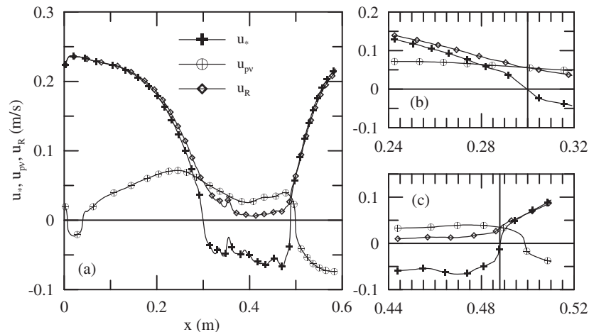
Fig. 1. Characteristic behaviour of u_* , u_{pv} and u_R for the flow of Na and Moin (1998). (a) Global behaviour, (b) behaviour near to the separation point, (c) behaviour near to the reattachment point.
