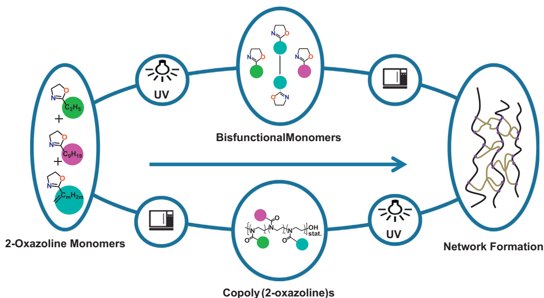
Scheme 1. Route 1 (top) and Route 2 (bottom) for the synthesis of crosslinked networks investigated in this study. 2-But-3'-enyl-2-oxazoline ( m = 3 ) and 2-Dec-9'-enyl-2-oxazoline ( m = 9 ) were used as olefinic monomers.
