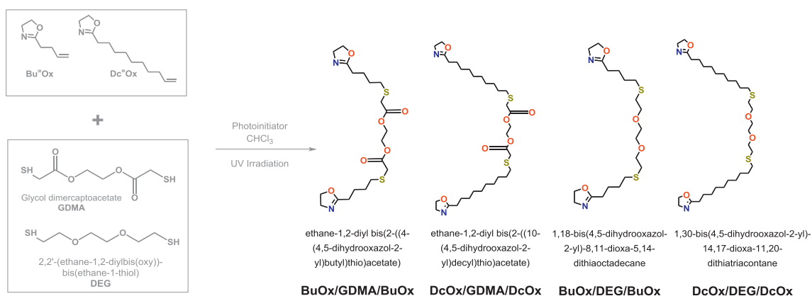
Scheme 2. Structures of the 2-oxazoline monomers investigated in this study.
