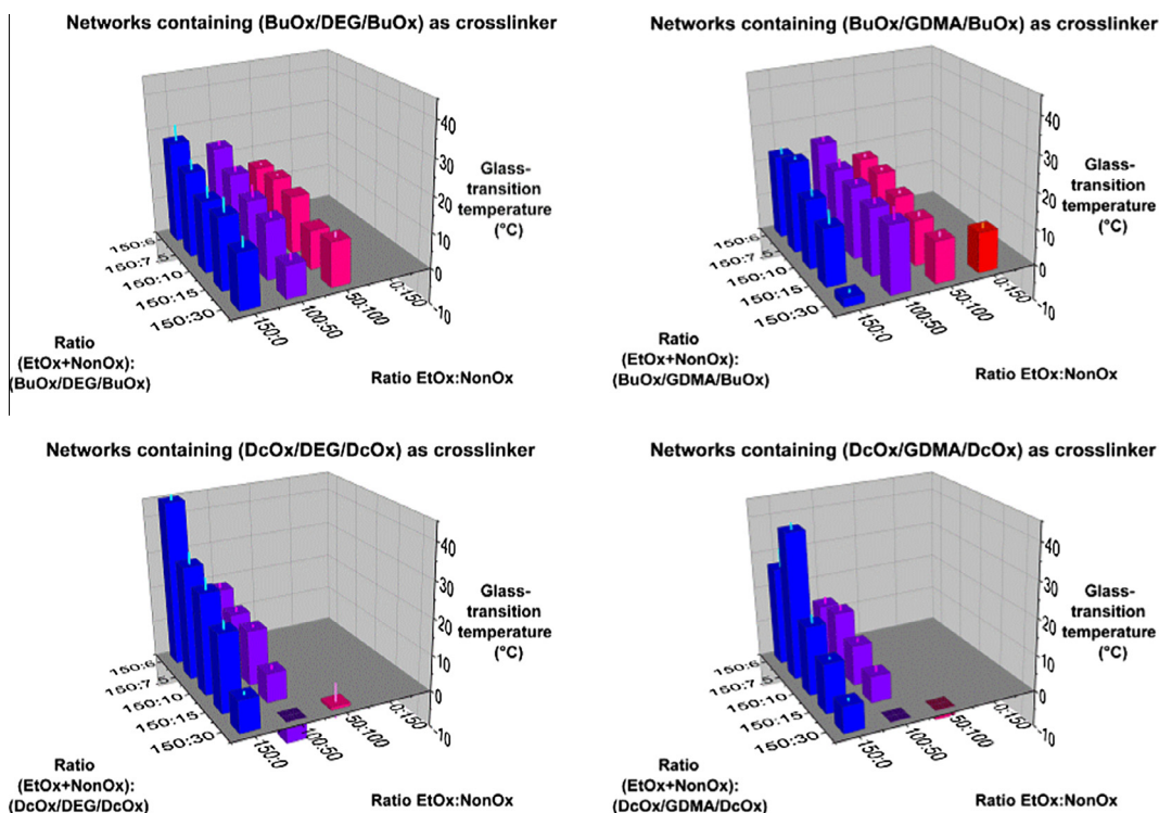
Fig. 1. Glass-transition temperatures of the copoly(2-oxazoline)-based networks.
