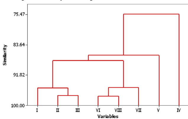
Figure 10 Dendrogram for the hierarchical clustering of different stations in the El-Mex Bay during the study period.
