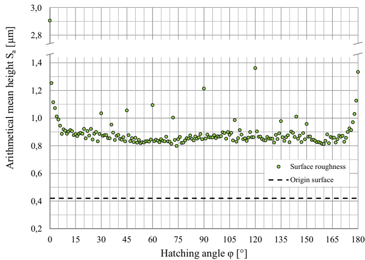
Fig. 2. Surface roughness depending on the hatching angle.
