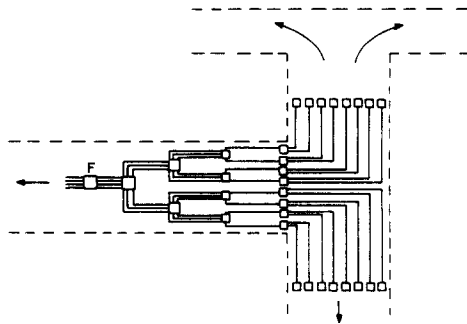
FIG. 8. An improved layout for the tree of meshes.
