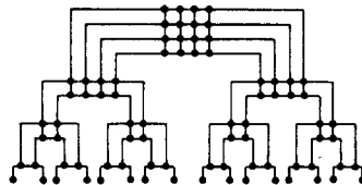
FIG. 5. The 4 \times 4 tree of meshes T_4 .
