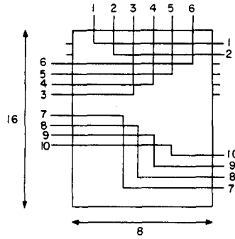
FIG. 6. Using a mesh in the tree of meshes as a crossbar switch.
