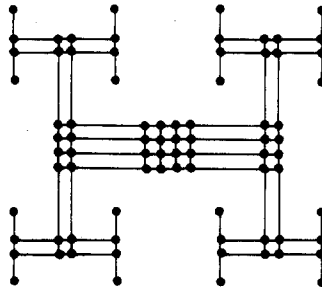
FIG. 7. The H -tree layout of the tree of meshes.
