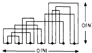
FIG. 2. Every N -node graph can be laid out in O(N^2) area.
