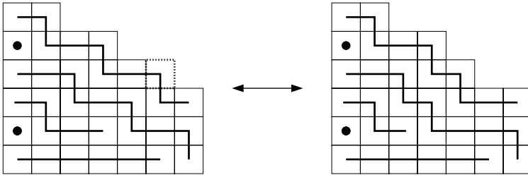
Fig. 5. Example of matching between (\alpha, \lambda) and (\beta, \lambda^-) for two flat pairs.
