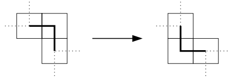
Fig. 4. Rerouting hooks to fit inside dg(\lambda^-) .
