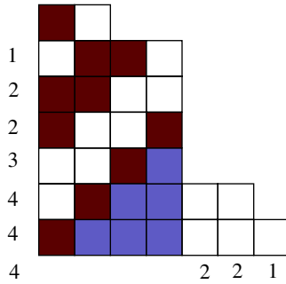
Fig. 7. Decomposition of \lambda = (7, 6, 4, 4, 4, 4, 2) .
