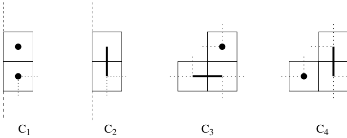
Fig. 2. Possible interactions between consecutive rim-hooks.
