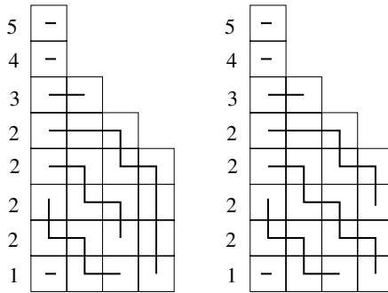
Fig. 3. Example of the involution \psi .
