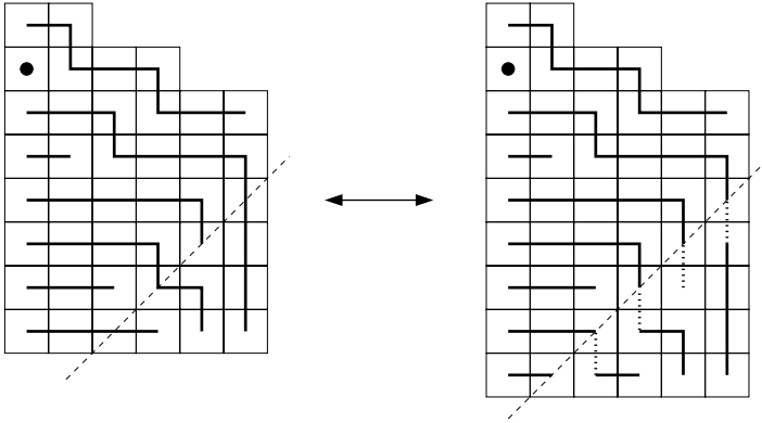
Fig. 6. Example of adding a new rim-hook along the bottom.
