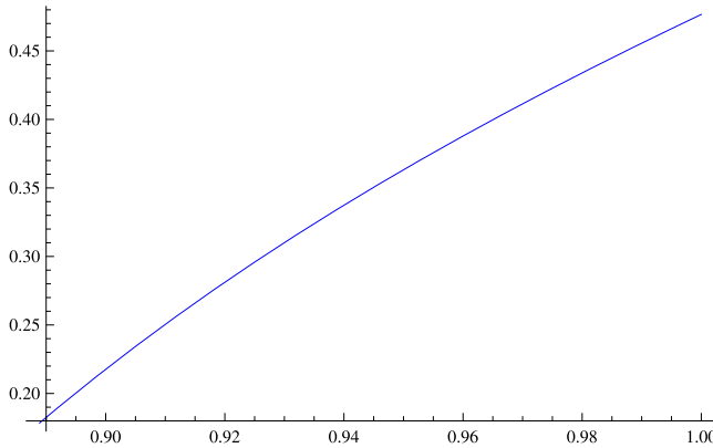
Fig. 1. Graph and select values of \tilde{C}(\theta) , 8/9 \leq \theta \leq 1 .
