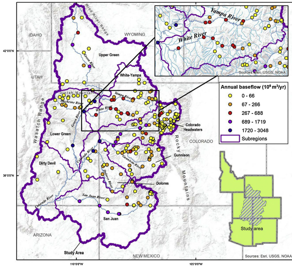
Fig. 1. Annual baseflow volumes for the UCRB and the White River watershed (subregions defined by HUC 4 boundaries).
