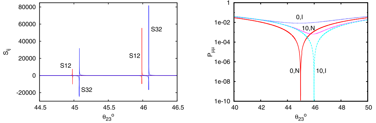
Fig. 1. (Left) The terms S_{12} and S_{32} as a function of \theta_{23} . The values on the left are for the normal hierarchy solution with \theta_{13} = 0 while those on the right are for the inverted hierarchy with \theta_{13} = 10^\circ . In both sets, the curves for S_{32} have been offset by \theta_{23} = 0.1^\circ for clarity, else the two curves for S_{12} and S_{32} would overlap each other. In the former case, \delta_{CP} = 0 and L/E = 611.165 km/GeV while for the latter, \delta_{CP} = 180^\circ and L/E = 604.629 km/GeV. (Right) The denominator P_{\mu\mu} plotted as a function of \theta_{23} for the same parameters. The dips as P_{\mu\mu} \rightarrow 0 correspond to the sharp peaks in S_{ij} on the left.
