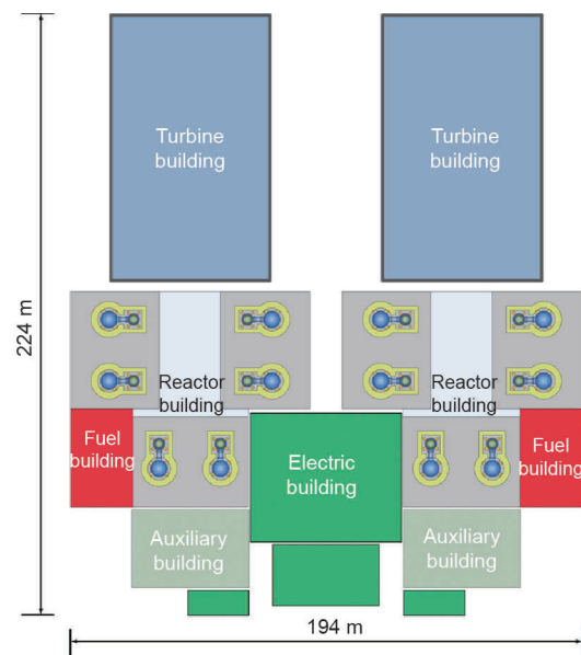
Fig. 6. The 2 × 600 MW e HTR-PM multi-modules plant.
