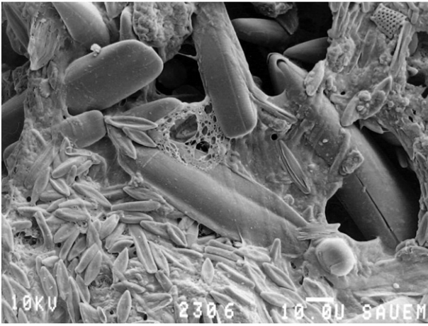
Fig. 8. EPS embedded microorganism within a biofilm: diatoms of various sizes that secrete polymeric substances to bind to each other and to sediment particles, thus enhancing sediment stability and impacting the whereabouts of non-polar ATCs. Low Temperature Scanning Microscopy LTSM image from the SERG laboratory of Prof. D.M. Paterson, image by I. Davidson, EU Marie Curie RTN project KEYBIOEFFECT.
