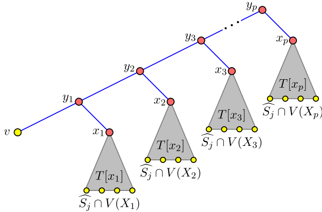
Fig. 1. Construction of T' .
