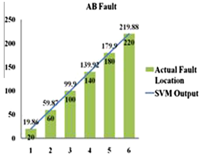
Fig. 11b. Actual versus predicted distance plot for AB fault.
