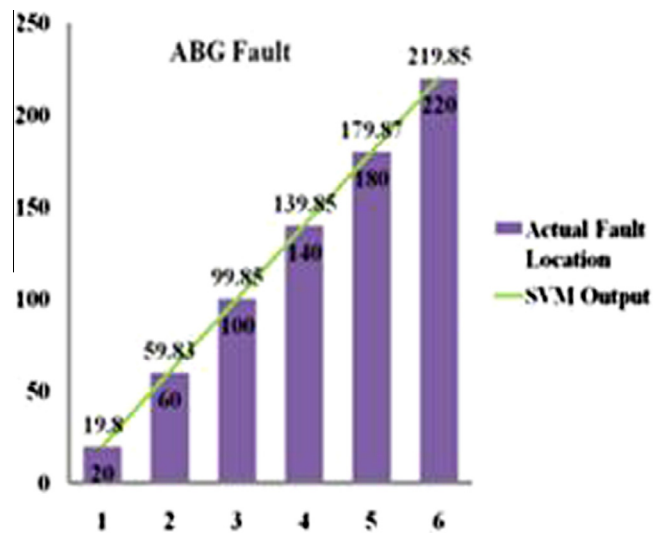
Fig. 11c. Actual versus predicted distance plot for ABG fault.
