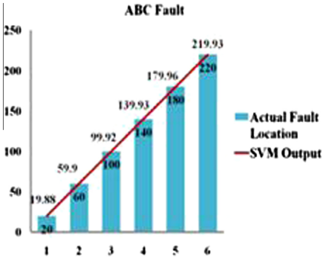
Fig. 11d. Actual versus predicted distance plot for ABC fault.
