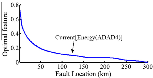
Fig. 9a. Optimal feature plot of coefficient ADAD4 of energy of current signal.
