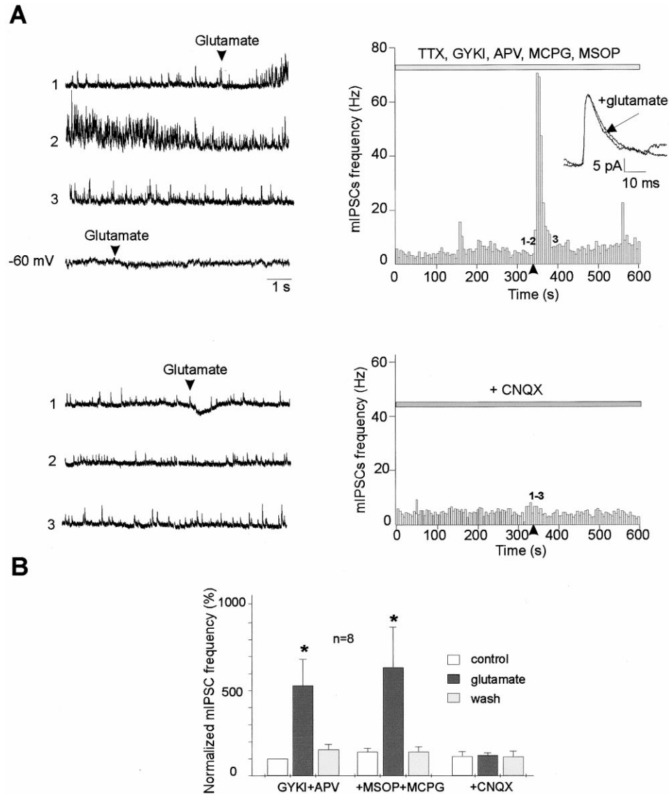
Figure 3. Bath Application of Glutamate Increases the Frequency of mIPSCs on Interneurons via the Activation of Kainate Receptors (A) Focal application of glutamate increases mIPSCs frequency in interneurons via the activation of kainate receptors. Puff application of glutamate (3 mM; 100 kPa for 50 ms) 50 \mu m away from the soma of the recorded interneuron (GYKI 53655 [30 \mu M], D-APV [50 \mu M], MCPG [500 \mu M], and MSOP [100 \mu M]) induced a large increase in the frequency of mIPSCs ( V_{\text{hold}} + 10 mV), as shown by the three consecutive trace recordings (1–3, top left) and frequency versus time plot histogram (top right). The amplitude and kinetics of the events are not changed by the application of glutamate, as shown by the superimposition of average traces ( n = 100 events averaged each). Miniature EPSCs ( V_{\text{hold}} - 60 mV) are totally suppressed in the presence of the blockers, and the same application of glutamate did not produce any current at the reversal potential for GABAergic events ( -60 mV). The effect of glutamate on mIPSCs is blocked when CNQX (50 \mu M) is added to the saline (see bottom traces and histogram). The small deflection of the baseline is most likely produced by the pressure applied close to the recording site. The recorded interneuron is an O-LM cell. (B) Pooled results for the effect of pressure-applied glutamate on mIPSCs in interneurons ( n = 8 cells). Pressure-applied glutamate in the presence of GYKI 53655 (30 \mu M) and D-APV (50 \mu M) significantly increased the frequency of mIPSCs ( p < 0.01 ). This effect is not prevented by addition of a cocktail of metabotropic glutamate receptor antagonists (MCPG [500 \mu M] and MSOP [100 \mu M]; p < 0.01 ), but it is completely prevented by addition of CNQX (50 \mu M). The bar graphs show mean \pm SEM values. * p < 0.01 .
