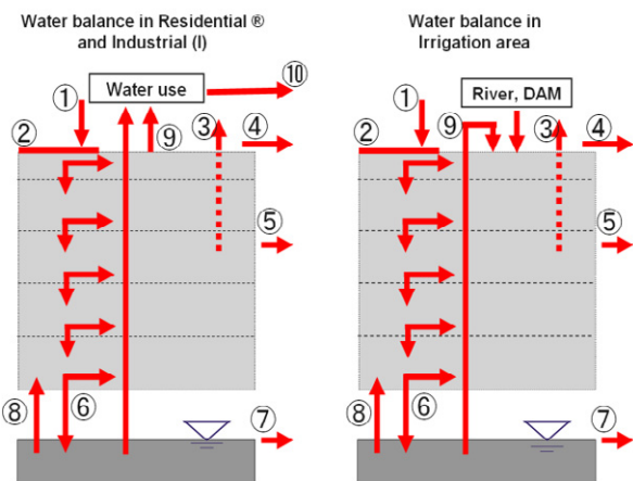
Figure. 2. Concepts of the proposed water management modeling in Chirchik river basin.
