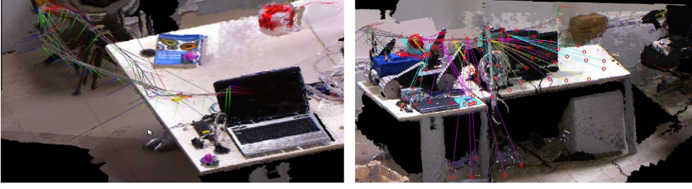
Fig. 7 Head poses of the subject during the experiment searching for the J , computed with the described localization algorithm, and the rays joining the head pose with the PORs (the red circles) projected on the scene point cloud. The lines represent, ideally, the intersection of the visual axes.
