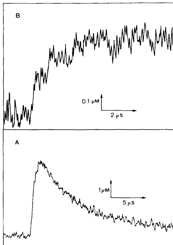
Fig.3. Transient protonation of bromothymol blue (A) and bromocresol green (B) by ground state 6-methoxyquinolinium. The solution of each dye ( 50 \mu\text{M} ) plus 2 mM 6-methoxyquinoline was photoexcited at a pH higher than the \text{p}K of the indicator. The dynamics of bromothymol blue was measured, at pH 8.3 ( \text{p}K = 7.0 ) and bromocresol green, at pH 6.4 ( \text{p}K = 4.95 ). Experimental conditions as in fig.2.
