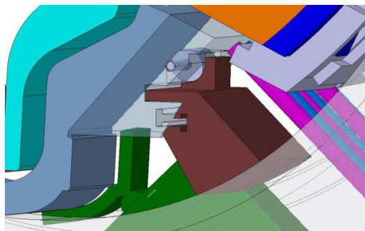
Fig. 8 Cam arrangement solution
