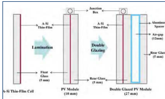
Fig 2. (a) Preparation for single plate of double-glazed PV module using transparent amorphous silicon (A-Si) thin-film cell; (b) specification property of thin film PV module.
