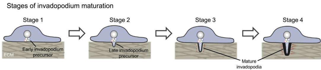
Fig. 1. Stages of invadopodium maturation. Stage 1 (early precursor stage): invadopodia initially form as non-degradative precursors that consist of a core structure containing actin, cortactin, cofilin, N-WASp, Tks5 and other proteins. Stage 2 (late precursor stage): kinases are activated, \beta 1 integrin and talin are recruited and Tks5 anchors the precursor to PI(3,4)P_2 . Stages 3–4 (mature invadopodium stage): in stage 3, actin polymerization is activated by stimulation of the NHE-1-cofilin pathway, and continued actin polymerization drives invadopodial elongation and stabilization. In stage 4, microtubule and intermediate filament recruitment facilitates further elongation of the protrusion, and matrix proteases are recruited to degrade the ECM (modified from Artym et al., 2006; Oser et al., 2009; Schoumacher et al., 2010; Sharma et al., 2013).
