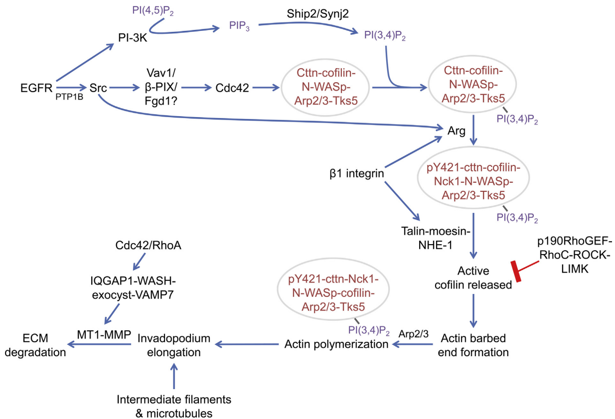
Fig. 2. Integrative signaling diagram of invadopodial assembly and maturation. Invadopodia initially form as precursors in response to EGF or other stimuli (e.g. TGF- \beta or PDGF). Src is activated either directly by EGFR or by PTP1B (Cortesio et al., 2008). These upstream signaling events induce Cdc42 activation, leading to assembly of the precursor core structure (red text within circle; Razidlo et al., 2014; Yamaguchi et al., 2005). The invadopodium precursor is then anchored by binding to PI(3,4)P 2 and further stabilized by \beta 1 integrin-mediated adhesion to the ECM (Beaty et al., 2013; Sharma et al., 2013). Invadopodium maturation begins as \beta 1 integrin activates Arg, which phosphorylates cortactin on Y421 to recruit Nck1 (Beaty et al., 2013; Oser et al., 2010). Talin localizes to the structure and recruits a complex of moesin and NHE-1 through a direct binding interaction with moesin (Beaty et al., 2014). The intracellular pH increases in response to NHE-1 activity, which disrupts the inhibitory interaction between cortactin and cofilin (Busco et al., 2010; Magalhaes et al., 2011). Cofilin severs F-actin to form barbed ends that are used to elongate filaments, on which Nck1 induces N-WASp-Arp2/3-dependent dendritic nucleation (DesMarais et al., 2004). Actin polymerization is required for MMP-dependent matrix degradation at invadopodia, possibly through MMP recruitment (Oser et al., 2009; Sakurai-Yageta et al., 2008; Yamaguchi et al., 2005). MT1-MMP is delivered by the IQGAP1-WASH-exocyst complex and fuses to the membrane via the v-SNARE VAMP7, resulting in matrix degradation (Monteiro et al., 2013; Sakurai-Yageta et al., 2008; Steffen et al., 2008). Cortactin, ctnn; synaptojanin2, synj2.
