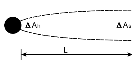
Fig. 3. Susskind's holographic screen.
