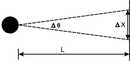
Fig. 1. When a light ray travels a distance L , the perpendicular direction obtains an uncertainty \Delta X . Equivalently, the direction of the light ray obtains an uncertainty \Delta\theta .
