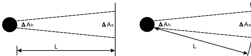
Fig. 4. Improved holographic screens. In the left figure, we illustrate the direct generalization of Susskind's holographic screen, which is planar. In the right figure, as Verlinde points out, we use an equipotential surface as a more natural choice of holographic screen.
