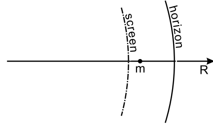
Fig. 2. To investigate the role that future event horizon plays in cosmology, we consider the setup as illustrated in the figure. The point m denotes a test particle located near the holographic screen.
