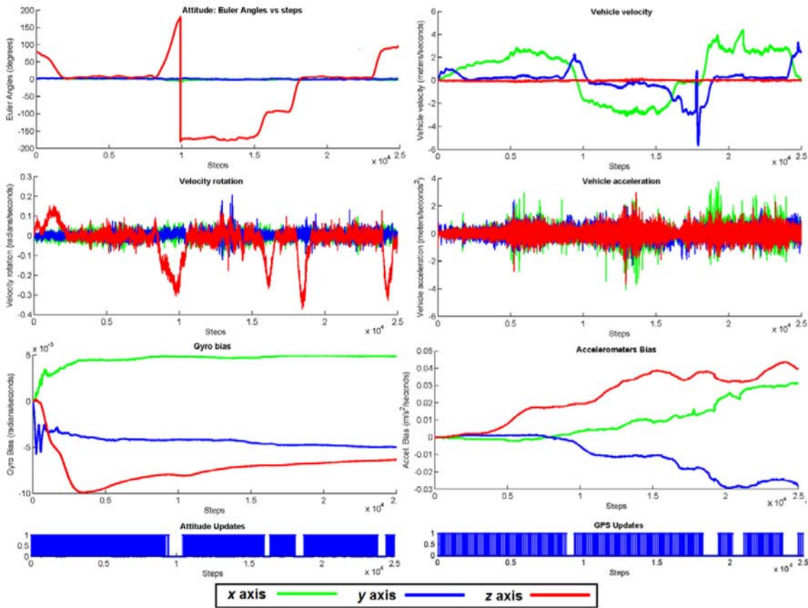
Figure 4. Estimation results for a) Attitude of the vehicle q^{nb} (expressed in Euler angles), b) Velocity of the vehicle v^n (expressed in the navigation frame n ), c) Gyroscopes bias x_g , d) Acceleration of the vehicle a^n (expressed in n ), and f) Accelerometers bias x_a . The lower plots illustrate periods where the attitude updates (left) and the GPS updates (right) occur.
