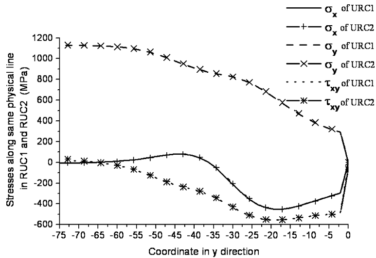
Fig. 8. The stress components along a same physical line AB in the same periodic structure (Fig. 7), from FEM analyses on two RUCs with different shapes.
