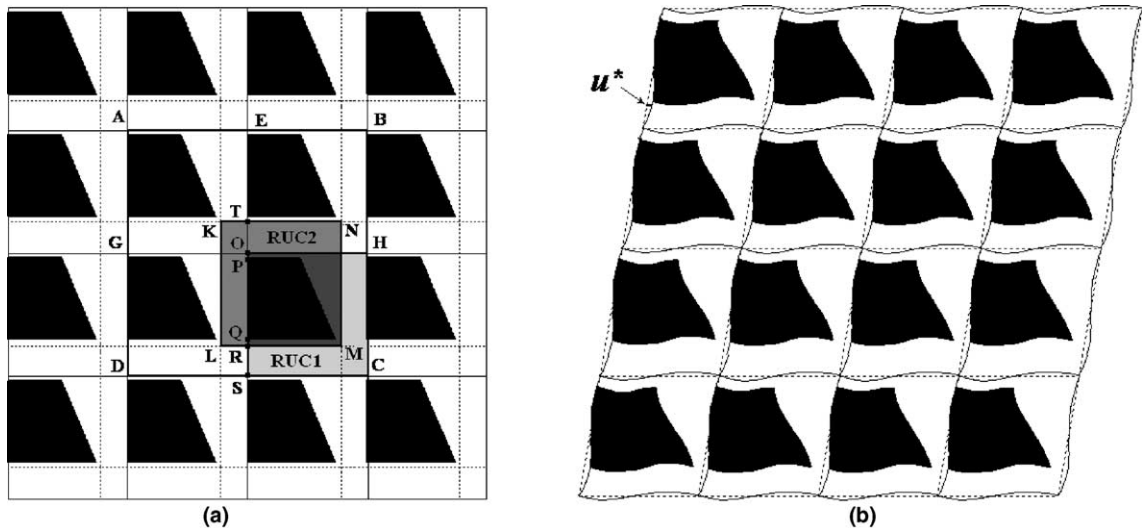
Fig. 1. A 2-D periodic structure without orthogonal axis of symmetry: (a) undeformed shape with two alternative choices of RUCs; (b) deformed shape under certain global load.
