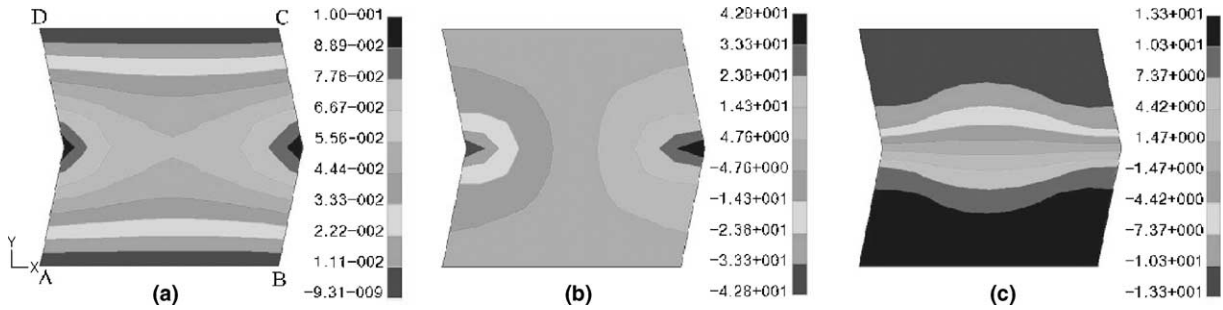
Fig. 2. A counter-example: a non-trivial solution which satisfies the trivial Eq. (9). (a) displacement \bar{u}_x ; (b) stress \sigma_x ; (c) stress \tau_{xy} .
