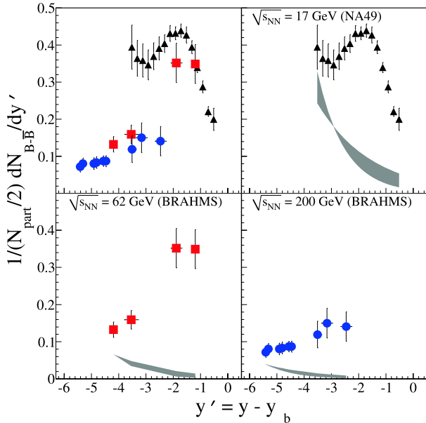
Fig. 4. The top left panel shows (1/N_{\text{part}}/2)dN_{B-\bar{B}}/dy' where y' = y - y_b for SPS and RHIC energies. No scaling is observed. The three other panels show data from SPS and RHIC drawn together with the ‘target’ net-baryon contribution from [21]. The triangles represent data from NA49, the squares BRAHMS data from 62 GeV and the circles BRAHMS 200 GeV data.
