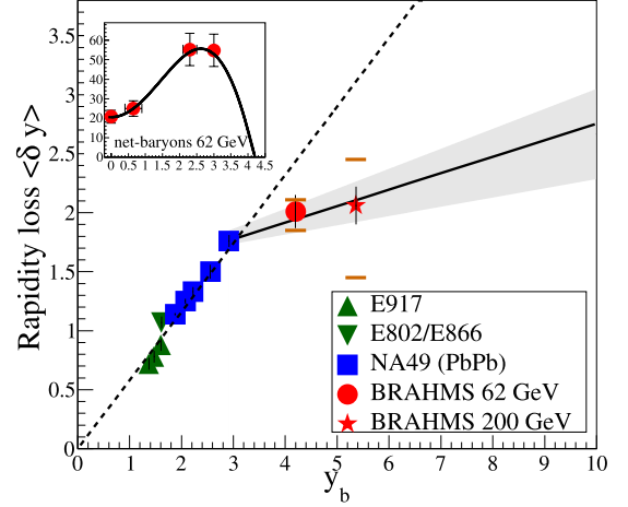
Fig. 3. Rapidity losses for heavy systems (Au,Pb) from AGS, SPS and RHIC as a function of beam rapidity. The solid line is a fit to SPS and RHIC data, and the band is the statistical uncertainty of this fit. The LHC beam rapidity is y = 8.67 . The dashed line is a linear fit to AGS and SPS data from [16]. The lower rapidity points from NA49 are preliminary data from [17].
