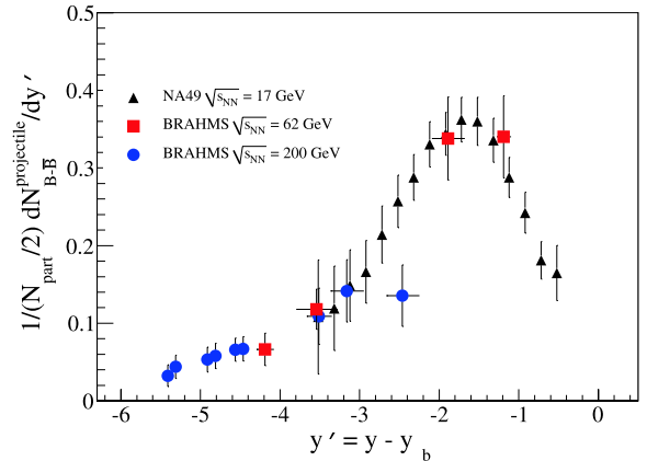
Fig. 5. Projectile net-baryon rapidity density (1/N_{\text{part}}/2)dN_{B-\bar{B}}^{\text{projectile}}/dy' from SPS and RHIC after subtraction of the target net-baryon contribution (see Fig. 4).
