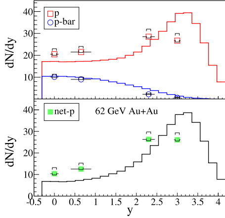
Fig. 2. Top: rapidity densities of protons and anti-protons. Bottom: rapidity densities of net protons. The statistical errors are smaller than the marker sizes. The vertical brackets shows the estimated systematic errors due the extrapolation of yields, and the horizontal bars indicate the width of the rapidity interval for each data point. The histograms are from HIJING/Bb(v2.1).
